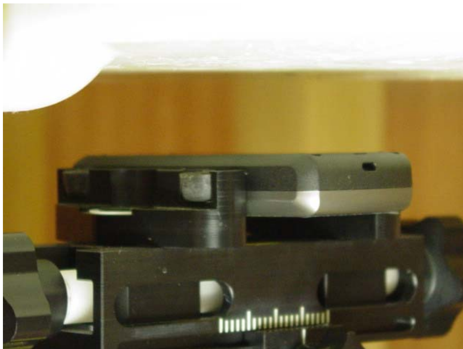
Figure 9E.3 Body SAR setup (22.5mm Air Separation)
