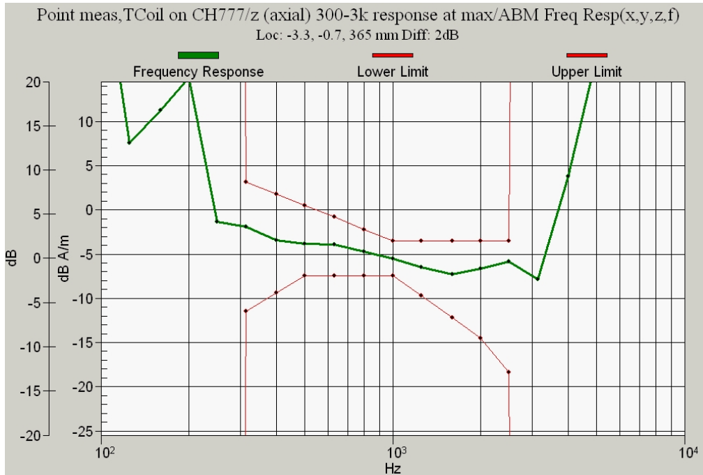
Figure 10.2c CDMA 800 Channel 777 Frequency Response
