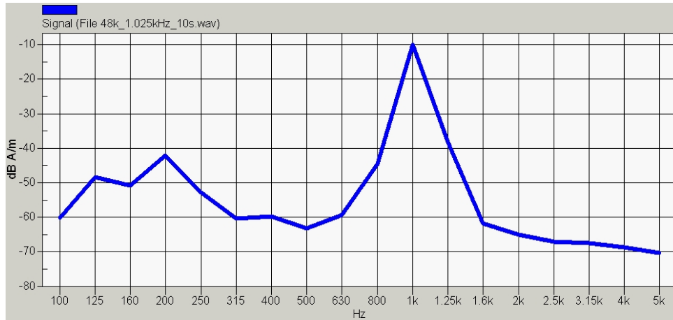
Figure 7.2a 1.025 KHz Voice signal spectrum
