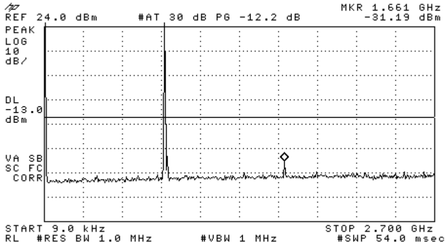
Figure 8-1a CDMA 800 – Conducted Spurious Emission (CH 1013)
