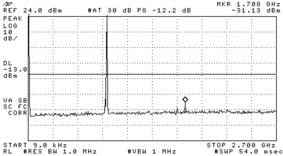
Figure 8-3a CDMA 800 – Conducted Spurious Emission (CH 777)
