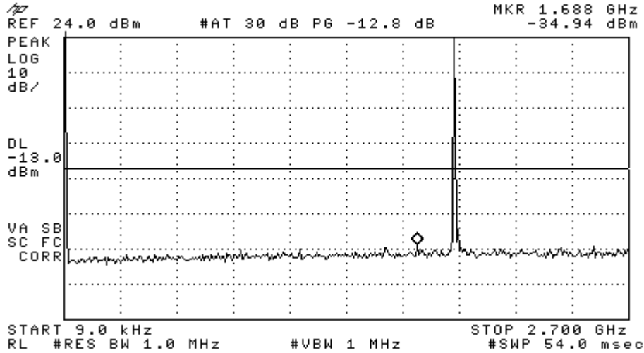
Figure 8-4a CDMA 1900 - Conducted Spurious Emission (CH 25)
