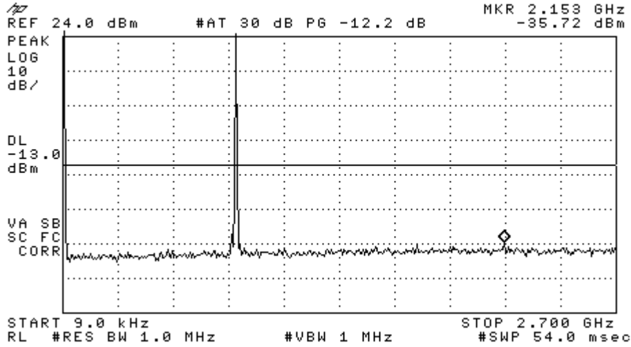
Figure 8-2a CDMA 800 – Conducted Spurious Emission (CH 383)
