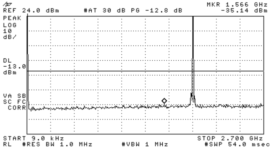
Figure 8-5a CDMA 1900 - Conducted Spurious Emission (CH 600)
