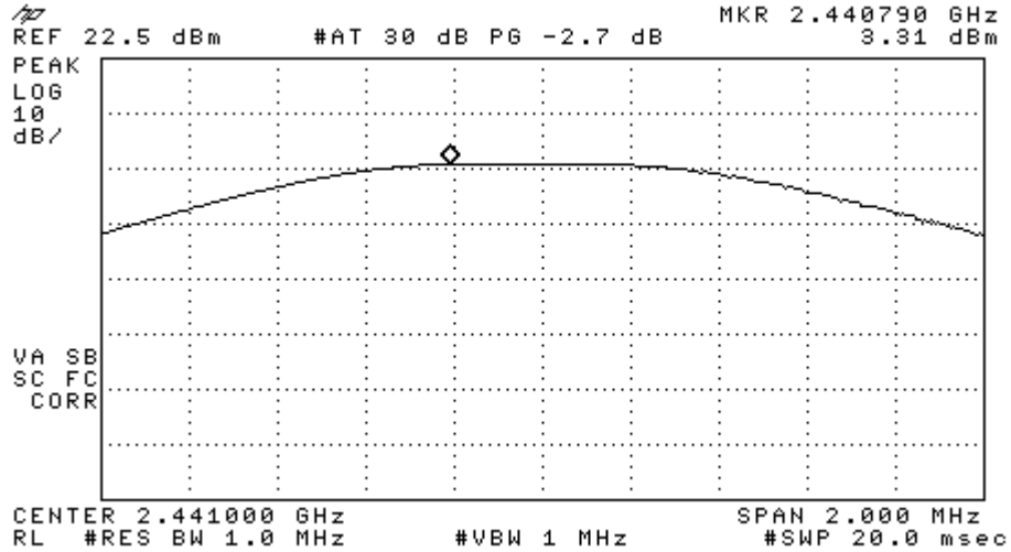
Figure 7b. Peak Output Power, Channel 39.
