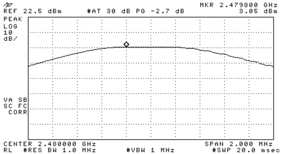
Figure 7c. Peak Output Power, Channel 78.
