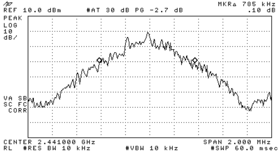
Figure 6b. 20 dB Bandwidth, Channel 39.
