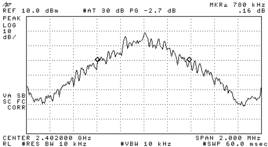
Figure 6a. 20 dB Bandwidth, Channel 0.
