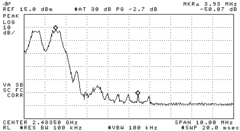
Figure 8-2b. High band edge with hopping enabled.
