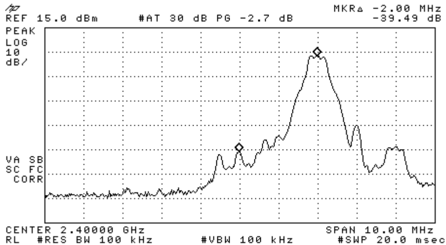
Figure 8-1a. Low band edge with hopping disabled.
