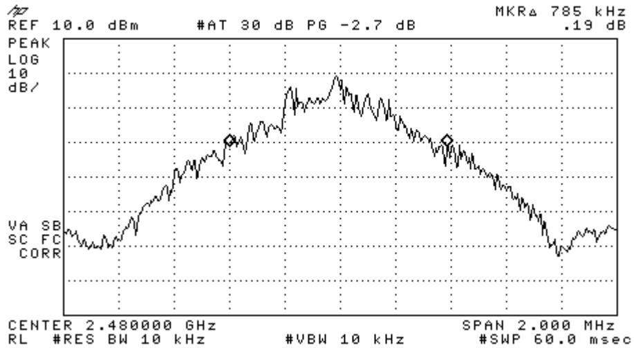
Figure 6c. 20 dB Bandwidth, Channel 78.
