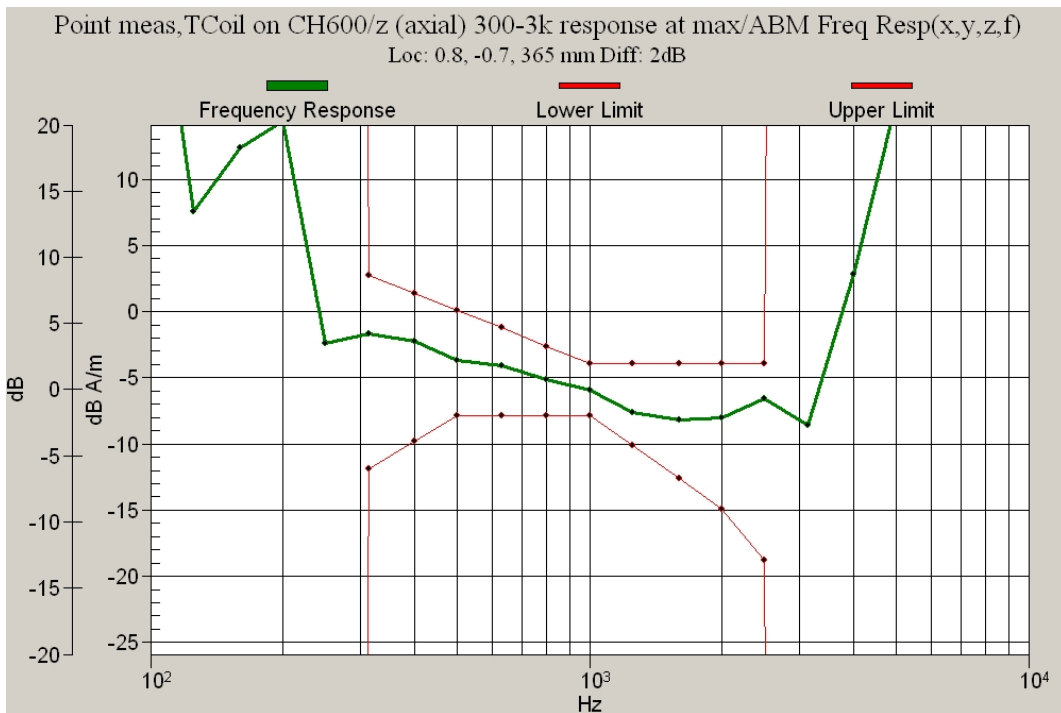
Figure 10.2e CDMA 1900 Channel 600 Frequency Response
