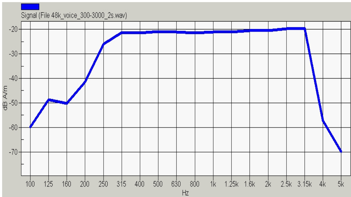
Figure 7.2b Broadband signal spectrum
