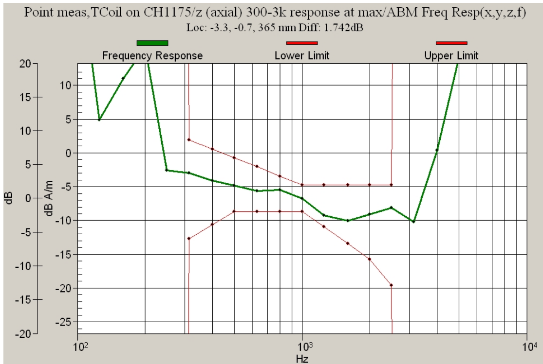
Figure 10.2e CDMA 1900 Channel 1175 Frequency Response
