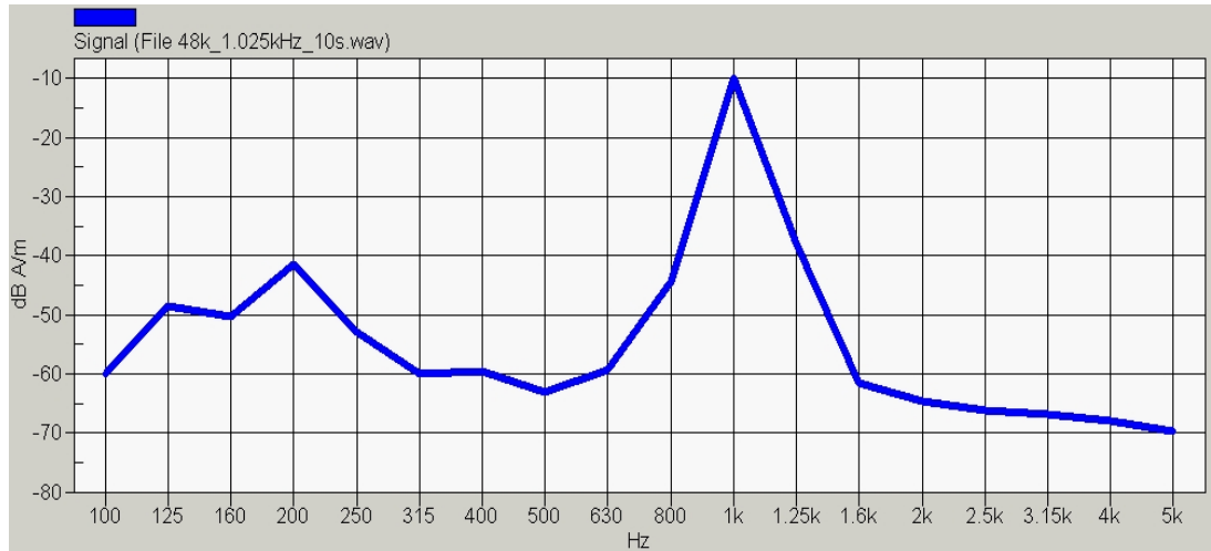
Figure 7.2a 1.025 KHz Voice signal spectrum
