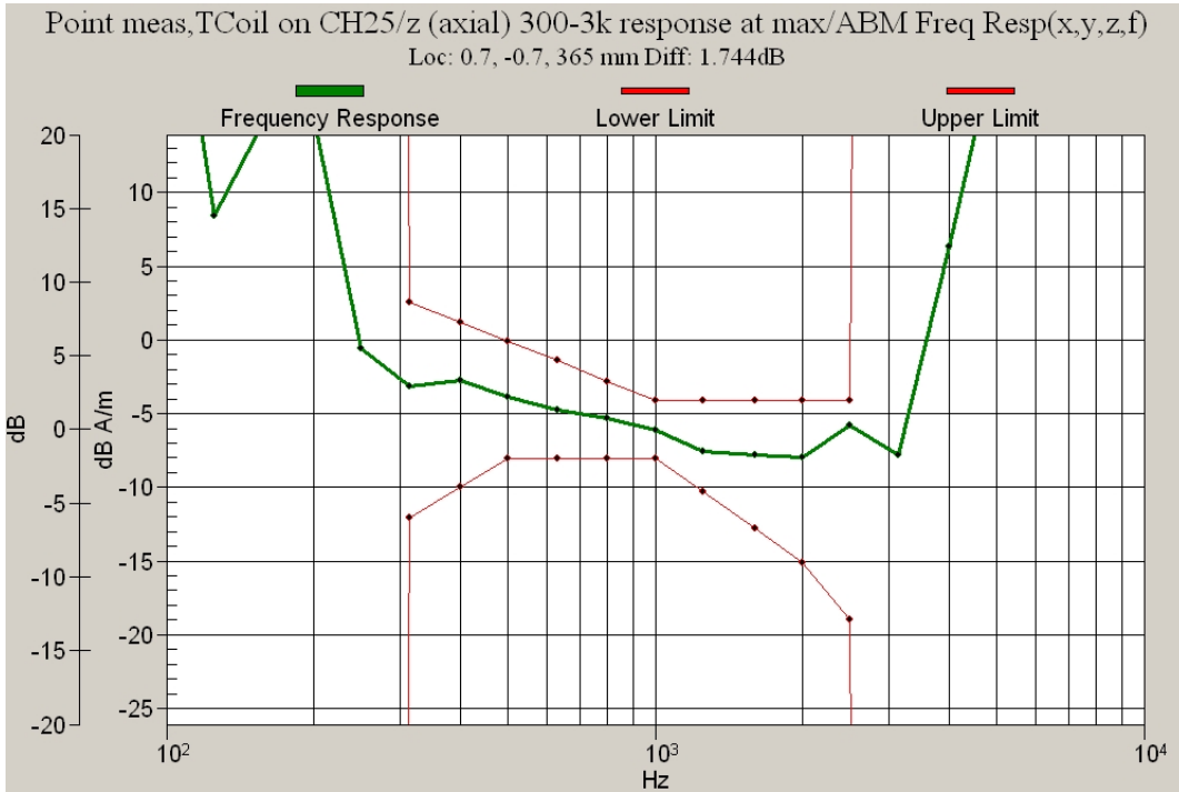
Figure 10.2d CDMA 1900 Channel 25 Frequency Response
