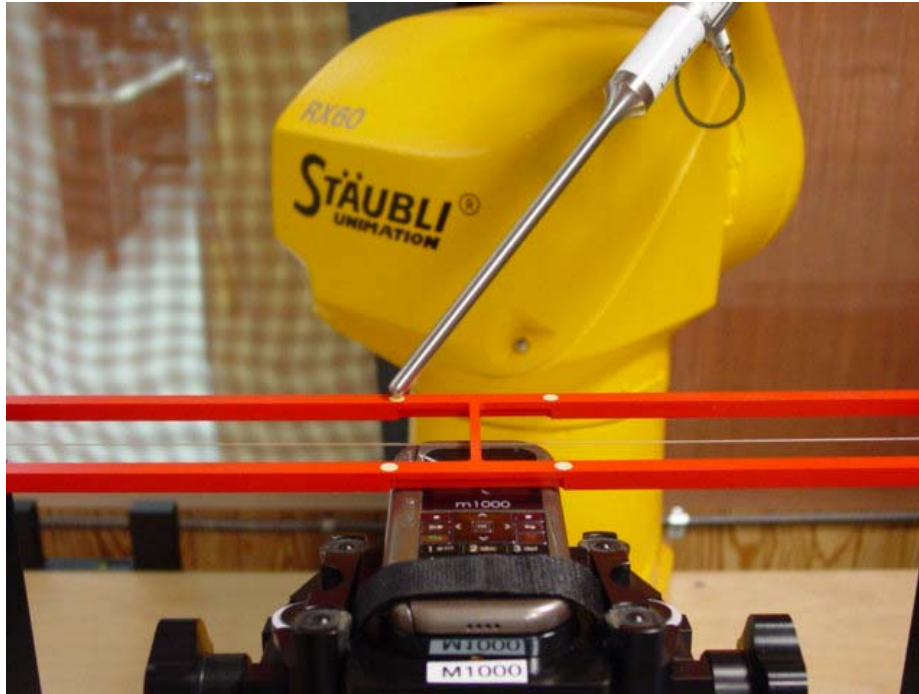
Figure 2 – HAC T-coil Test Setup
