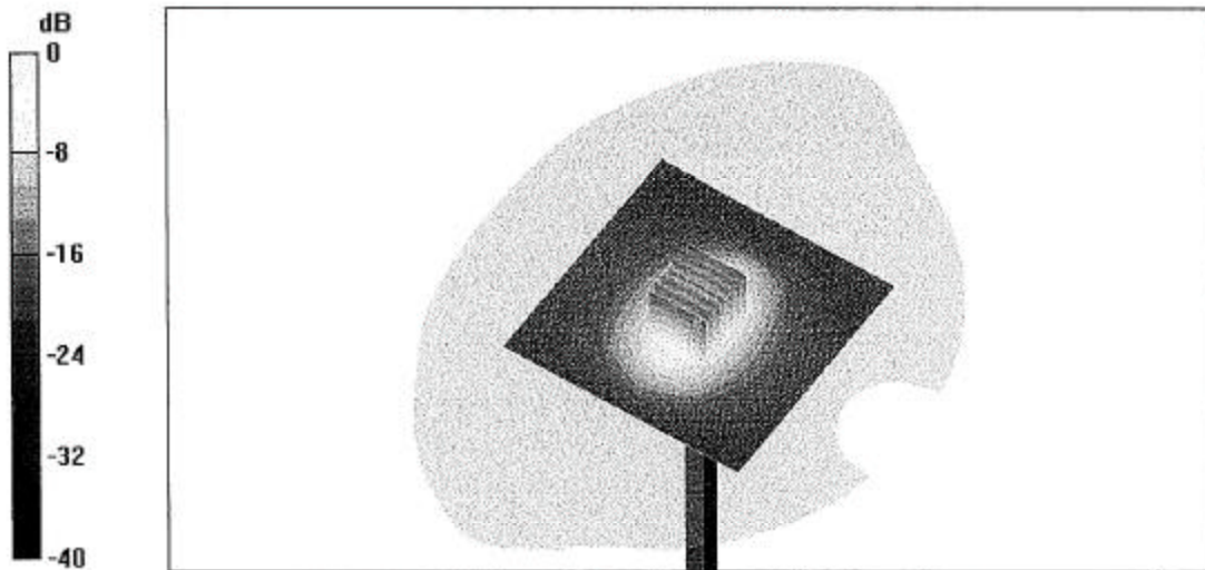
0 dB = 11.9mW/g
