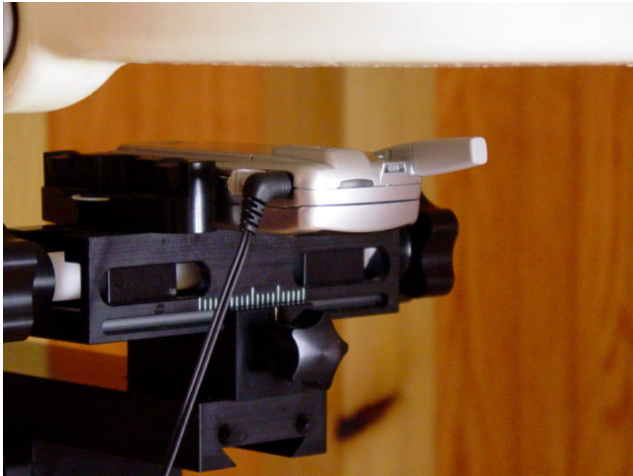
Figure 12.4 body SAR setup (with 25mm air separation)
