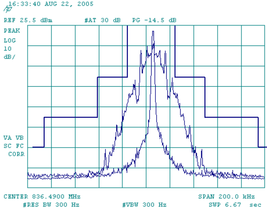
Figure 7-7 AMPS WIDEBAND
