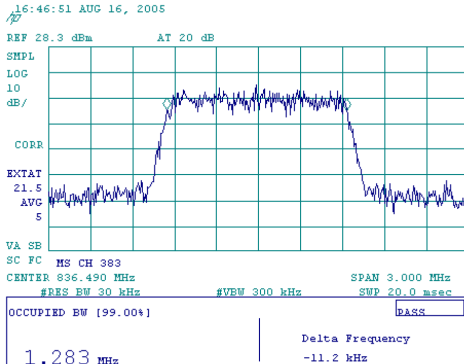
Figure 7-8 CDMA 800 @ CH 383
