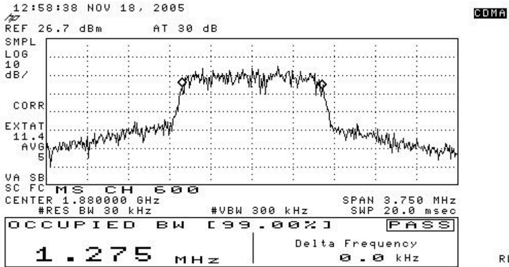
Figure 7-9 CDMA 1900 @ CH 600
