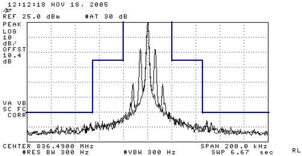
Figure 7-2 AMPS SAT
