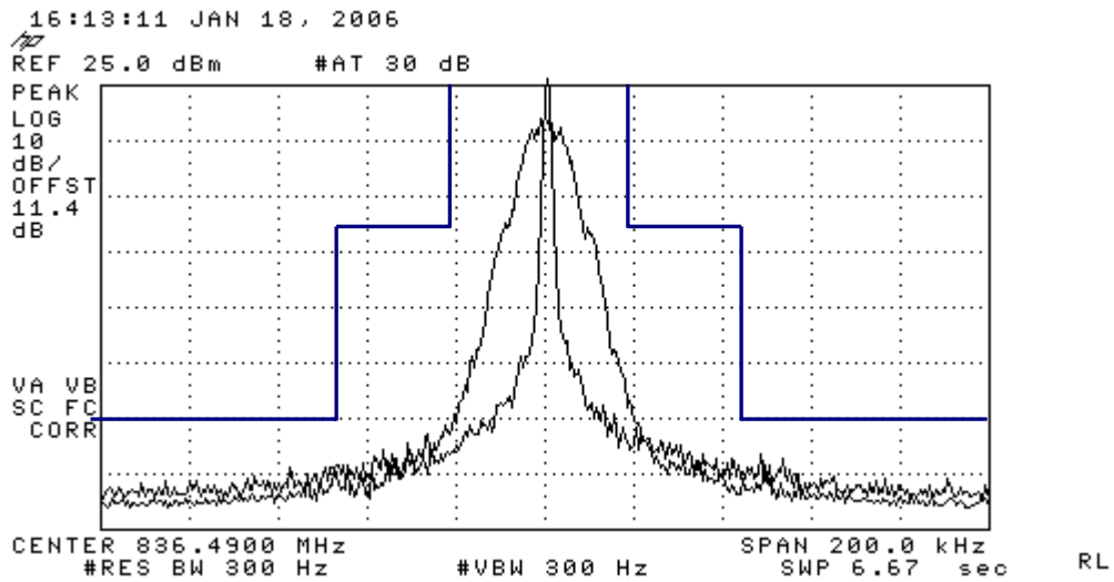
Figure 7-6 SAT + DTMF_9
