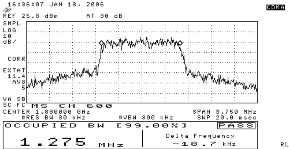
Figure 7-9 CDMA 1900 @ CH 600
