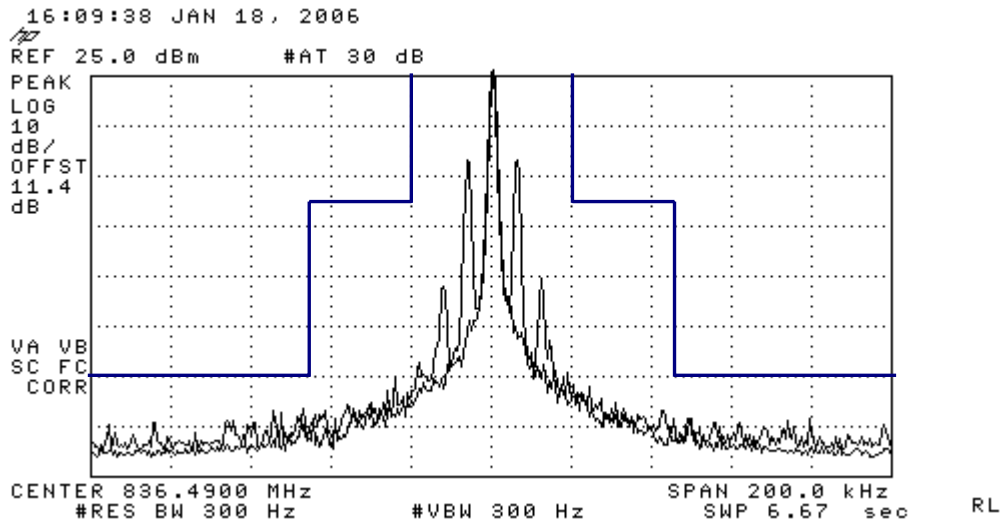
Figure 7-2 AMPS SAT
