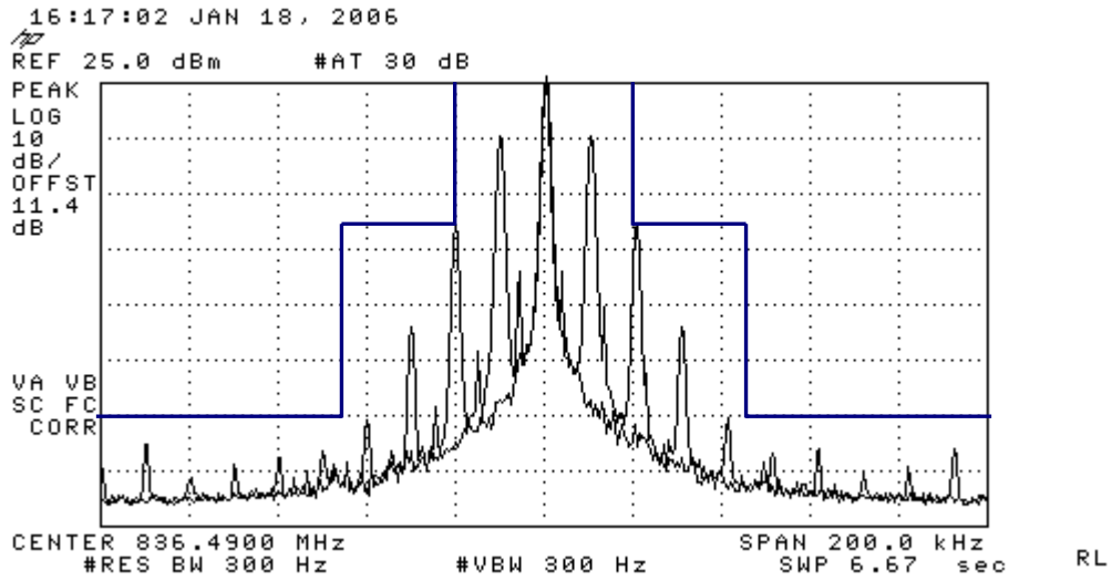
Figure 7-4 AMPS ST
