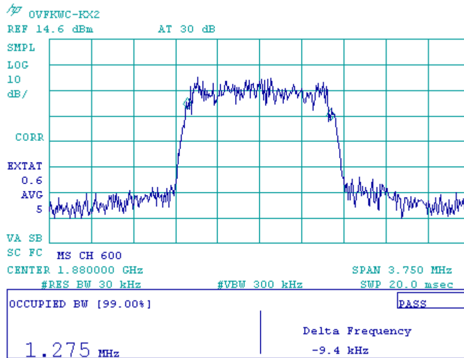
Figure 8-11 CDMA 1900 at RC1
