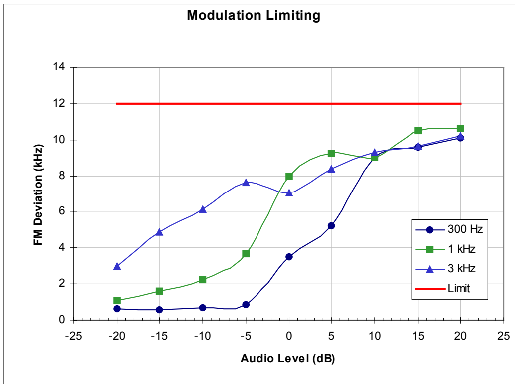
Figure 7.3 Modulation Deviation Limiting
