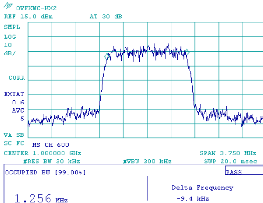
Figure 8-12c CDMA 1900 1X at RC3 (F/R-FCH)
