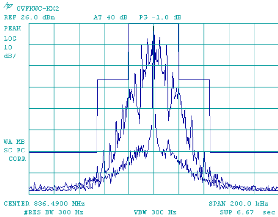
Figure 8-7 AMPS WIDEBAND
