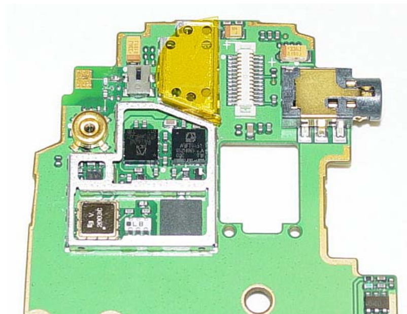
Main PCB_B without Shield & Camera
