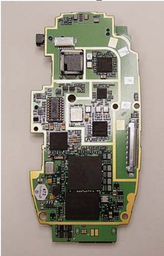
Main PCB_A
