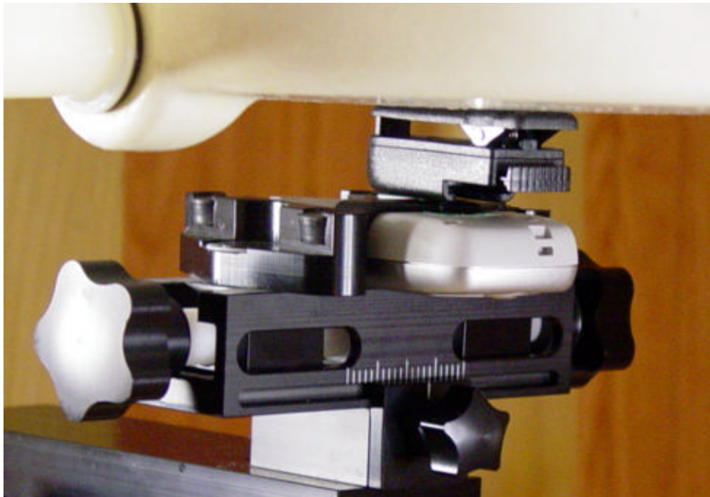
Figure 12.5 Body SAR Set-up (with phone clip)
