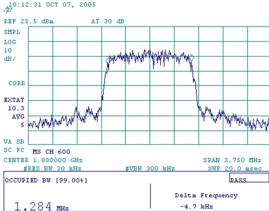
Figure 7-9 CDMA 1900 @ CH 600
