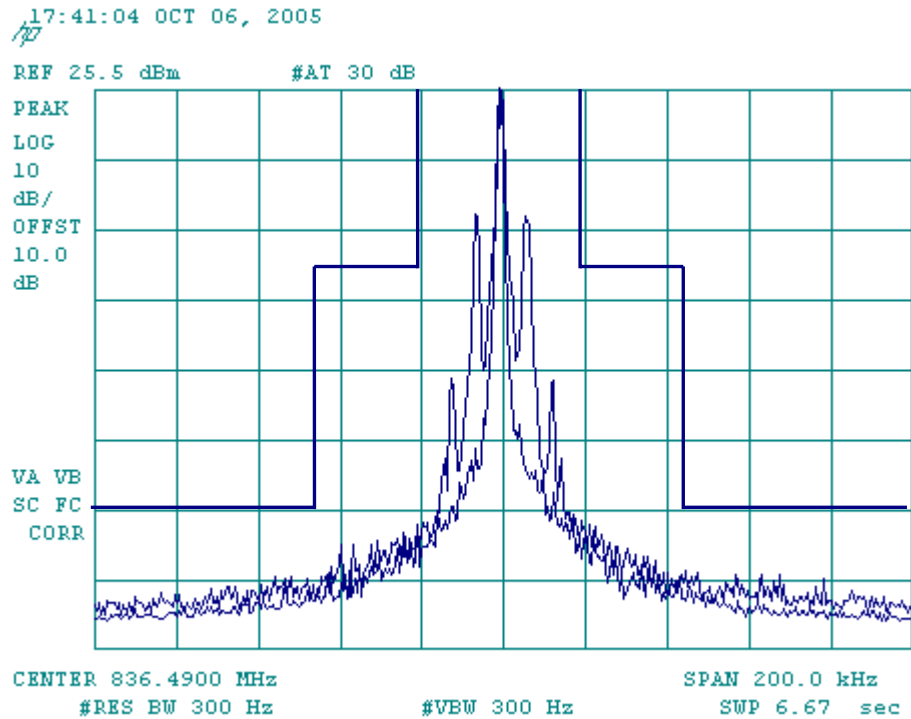
Figure 7-2 AMPS SAT
