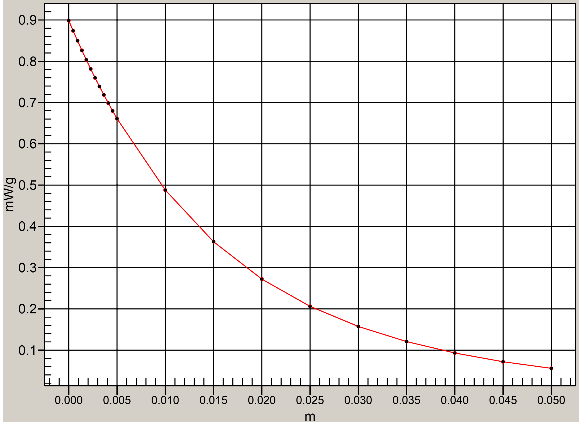
Interpolated SAR(x,y,z,f0) CDMA-800 RIGHT/Z Scan/Value Along Z, X=0, Y=0 SAR
