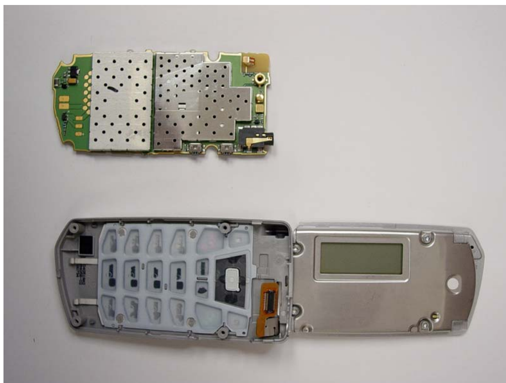
Lower-Half Assembling _ 1
