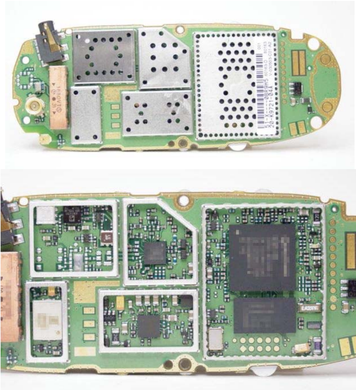
KE414 PCB side 1
