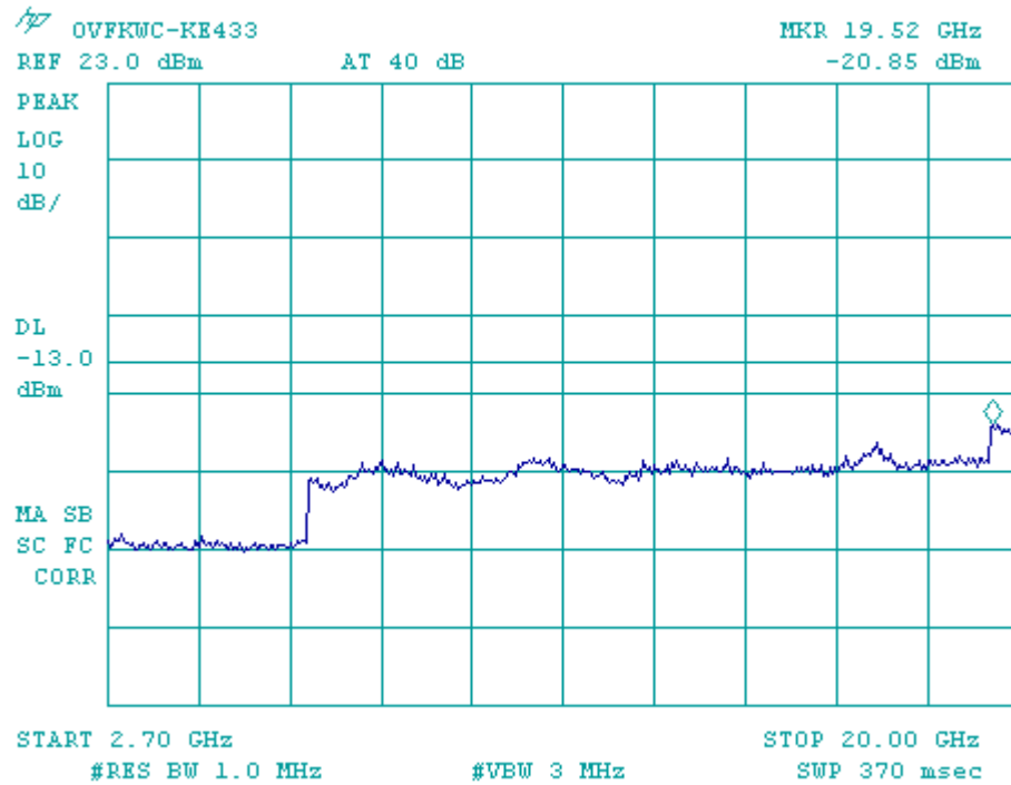
Figure 8-2b CDMA 1900 - Conducted Spurious Emission (CH 600)
