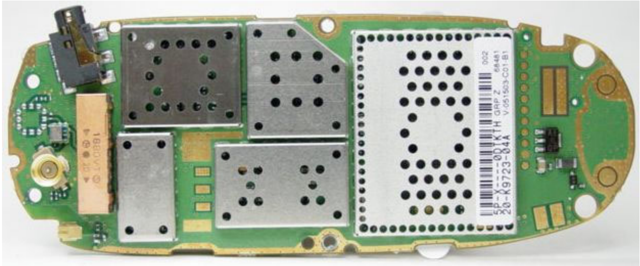
PCB side 1
