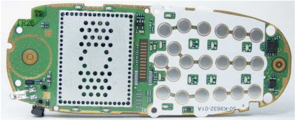
PCB Side 2
