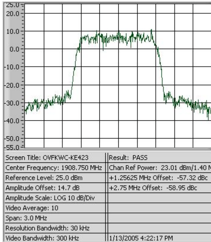
Figure 7-4 CDMA 1900 Upper Band Edge
