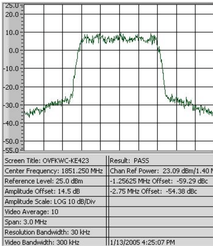
Figure 7-3 CDMA 1900 Lower Band Edge
