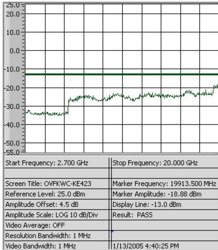
Figure 8-1b CDMA 1900 - Conducted Spurious Emission (CH 25)
