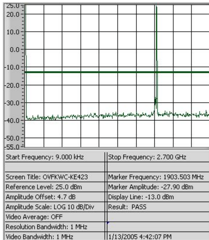
Figure 8-3a CDMA 1900 - Conducted Spurious Emission (CH 1175)
