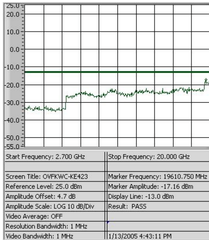
Figure 8-2b CDMA 1900 - Conducted Spurious Emission (CH 600)
