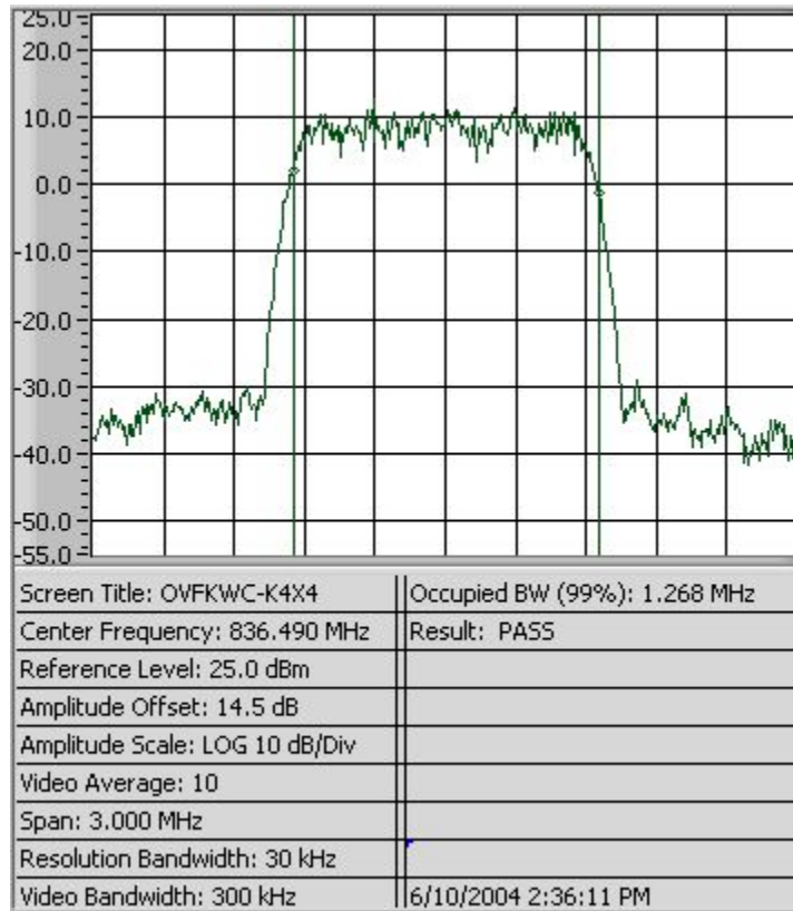
Figure 8-9 CDMA 800 1X at RC3
