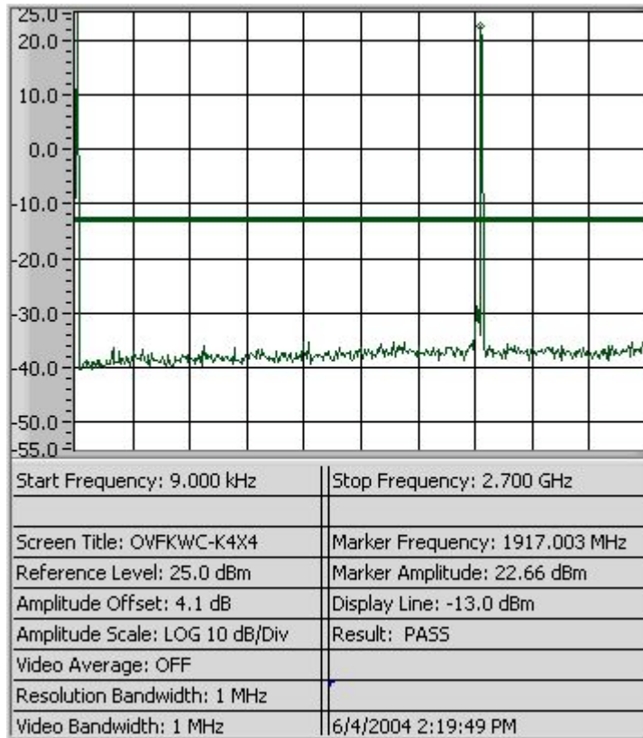
Figure 9-15a CDMA 1900 - Conducted Spurious Emission (CH 1175)
