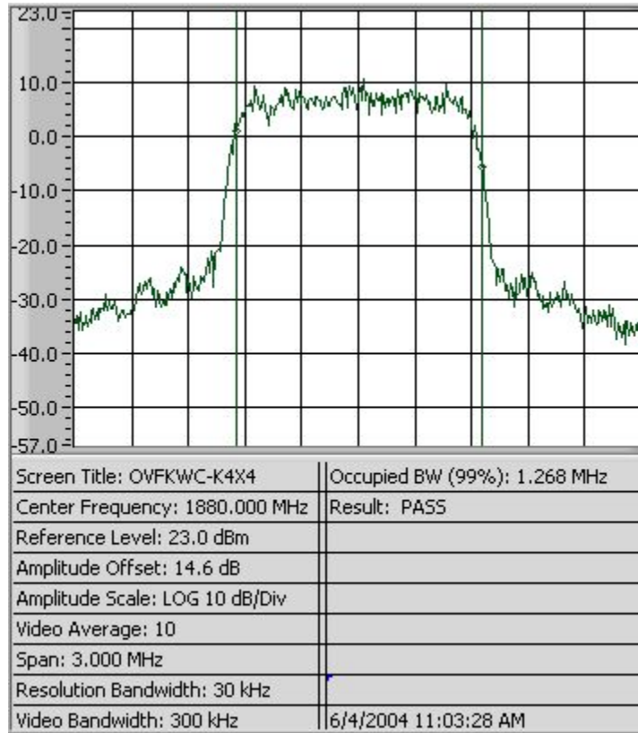
Figure 8-11 CDMA 1900 1X at RC3
