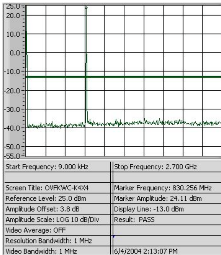
Figure 9-2a AMPS – Conducted Spurious Emission (CH 991)
