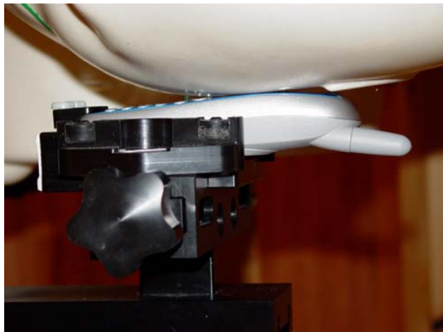
Figure 11.2 phone against the head (left cheek position)
