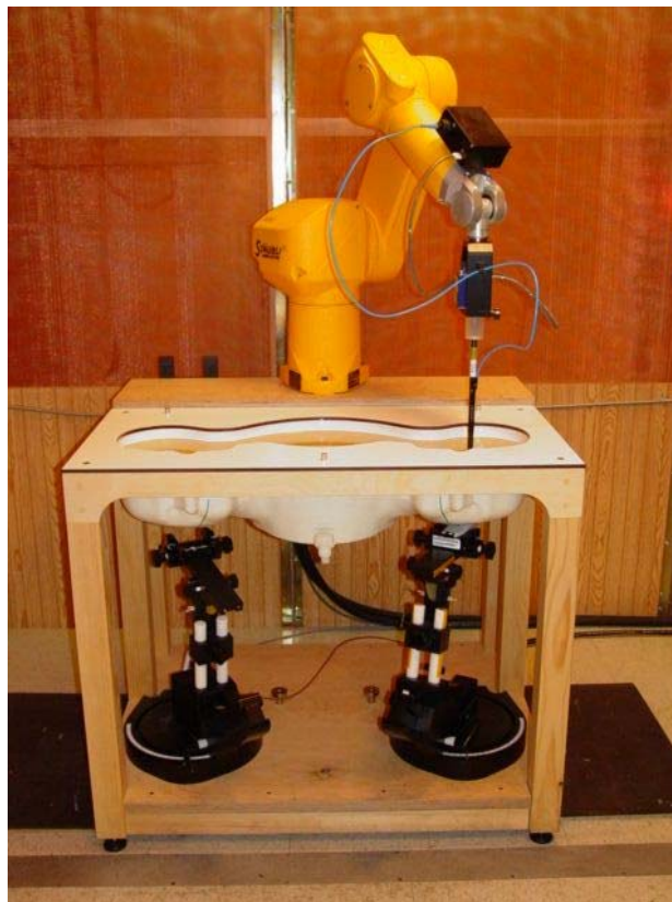
Figure 7.1 DASY 4 System
