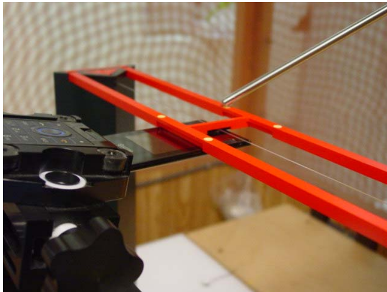
Figure 1b – HAC T-Coil Test Setup
