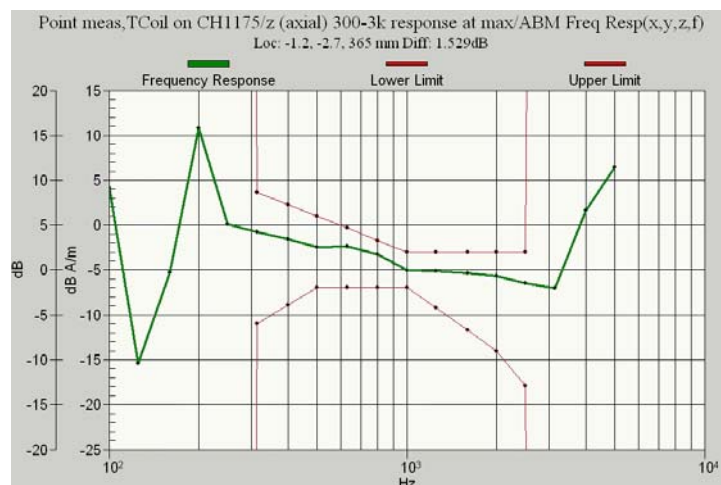
Figure 10.2e CDMA 1900 Channel 1175 Frequency Response
