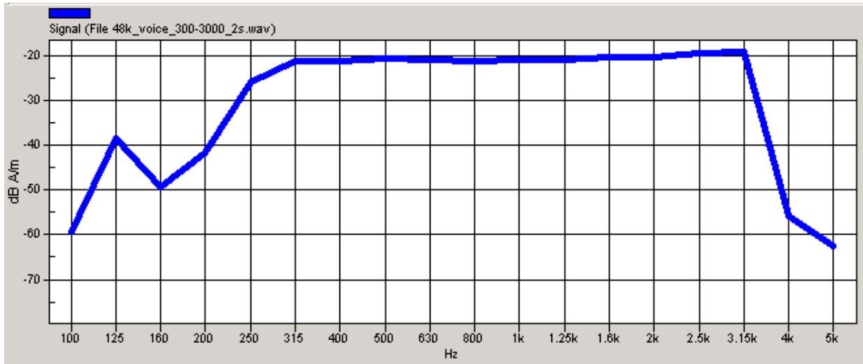
Figure 7.2b Boardband signal spectrum
