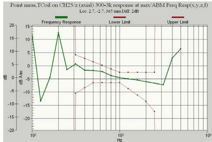
Figure 10.2d CDMA 1900 Channel 25 Frequency Response
