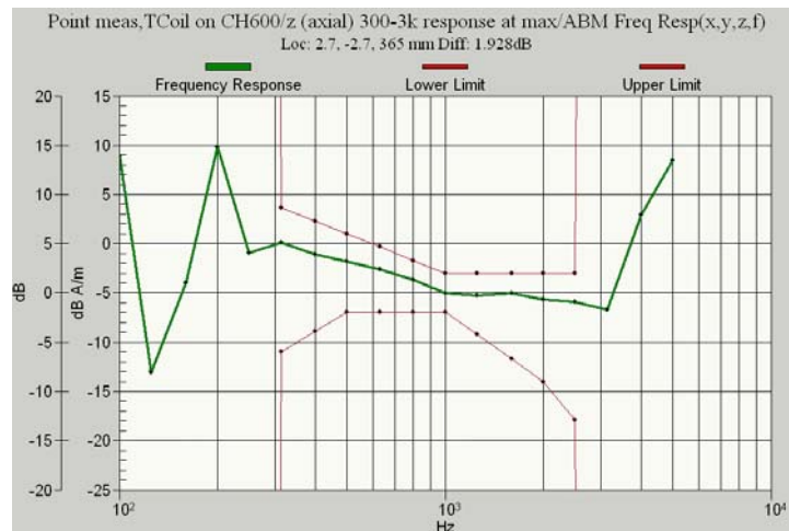
Figure 10.2e CDMA 1900 Channel 600 Frequency Response
