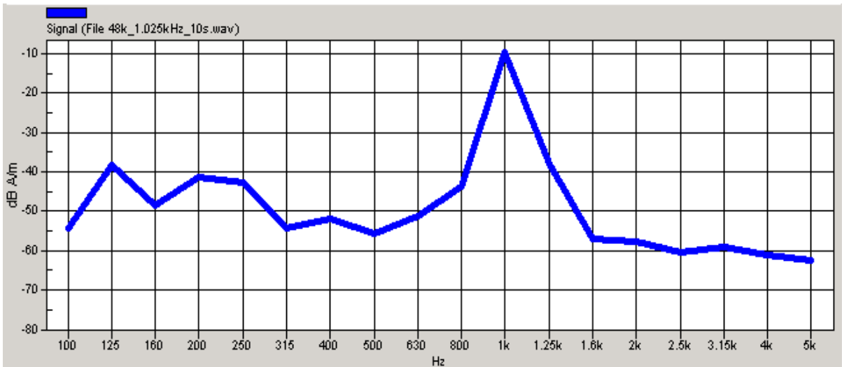
Figure 7.2a 1.025 KHz Voice signal spectrum
