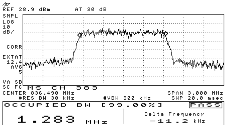
Figure 7-1 CDMA 800 @ CH 383
