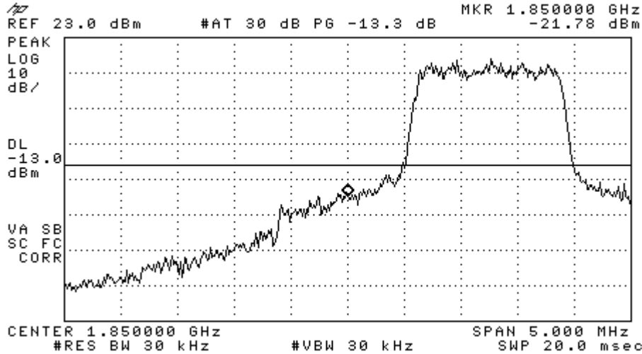
Figure 7-5 CDMA 1900 Lower Band Edge @ CH 25
