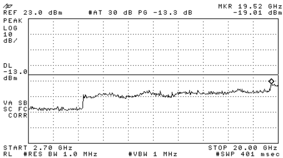
Figure 8-4b CDMA 1900 - Conducted Spurious Emission (CH 25)
