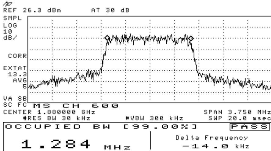
Figure 7-4 CDMA 1900 @ CH 600
