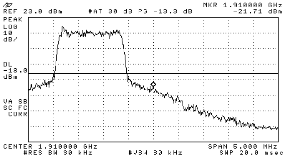
Figure 7-6 CDMA 1900 Upper Band Edge @ CH 1175
