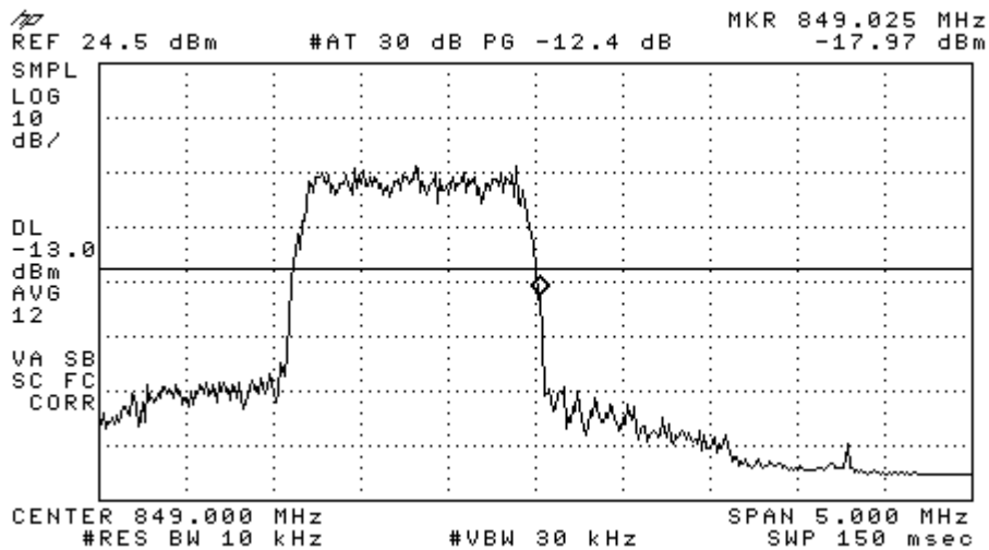
Figure 7-3 CDMA 800 Upper Band Edge @ CH 777
