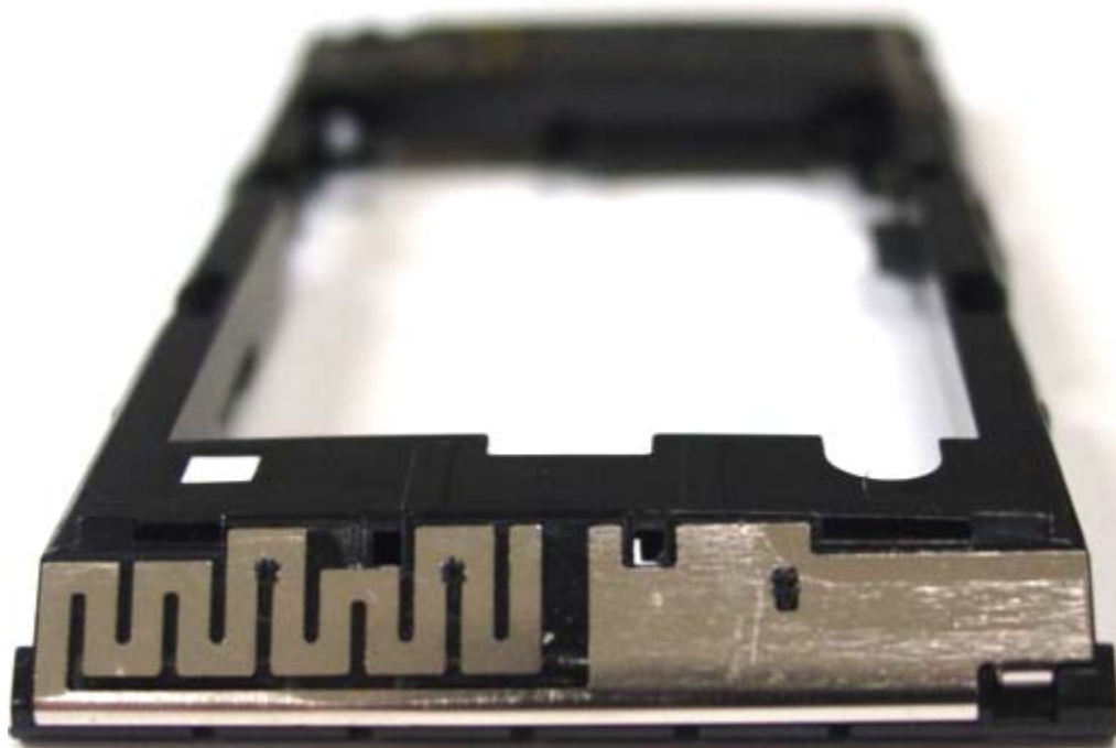
Original antenna - Close Up
