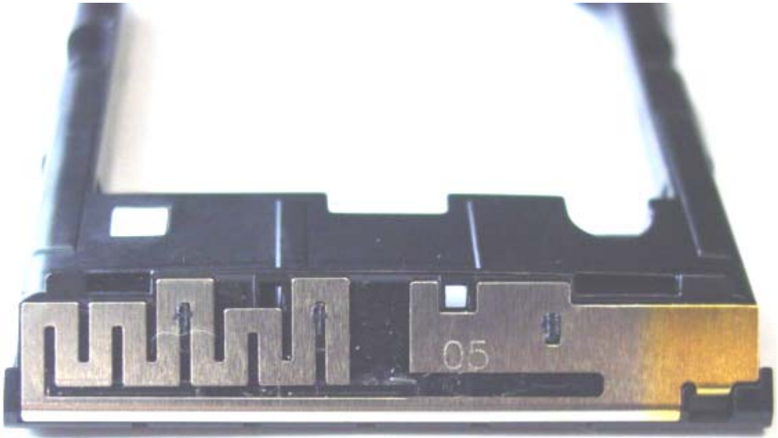
Modified Antenna – Close Up
