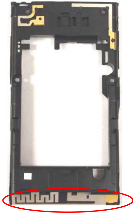
Modified Antenna
