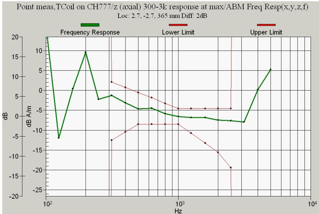
Figure 10.2c CDMA 800 Channel 777 Frequency Response
