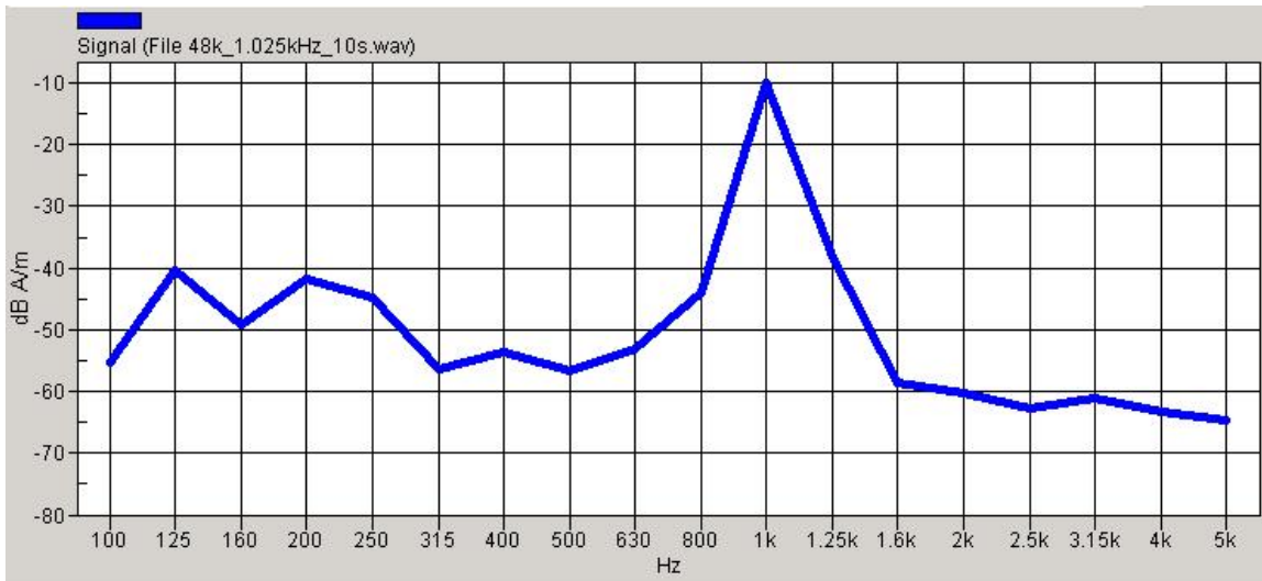
Figure 7.2a 1.025 KHz Voice signal spectrum
