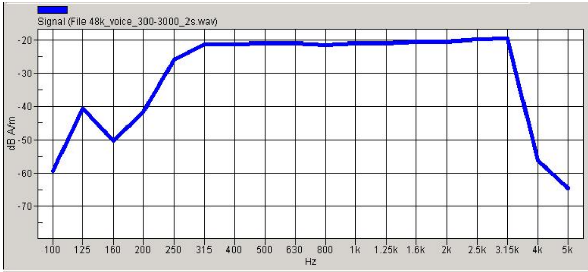
Figure 7.2b Boardband signal spectrum
