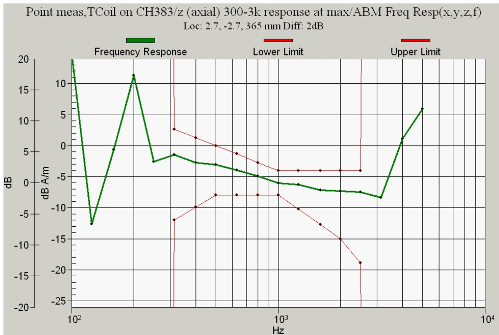
Figure 10.2b CDMA 800 Channel 383 Frequency Response
