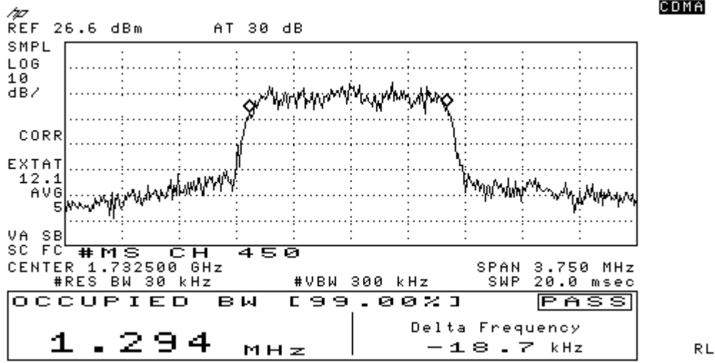
Figure 7-7 AWS 1700 @ CH 450
