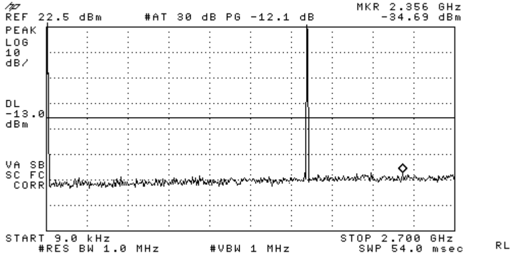
Figure 8-7a AWS 1700 - Conducted Spurious Emission (CH 25)
