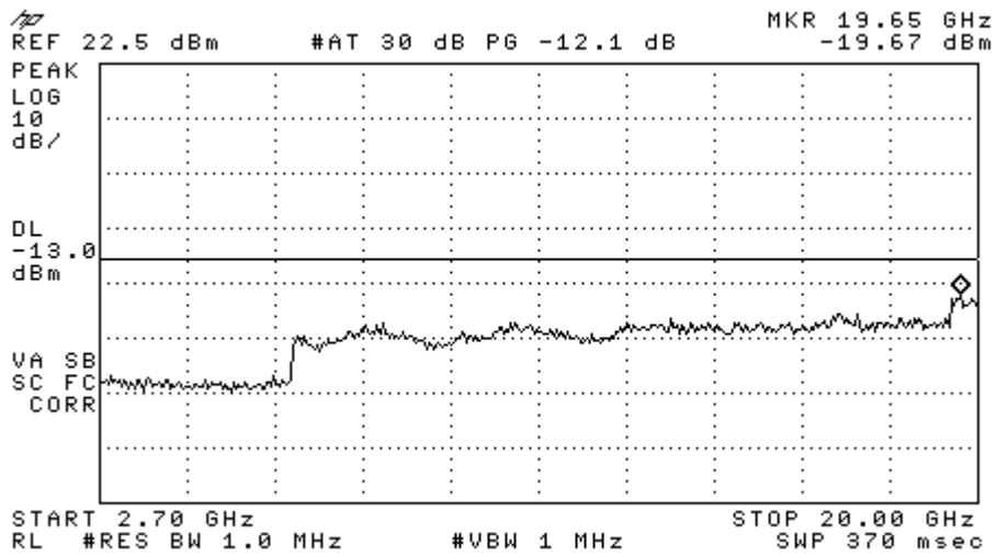
Figure 8-9b AWS 1700 - Conducted Spurious Emission (CH 875)
