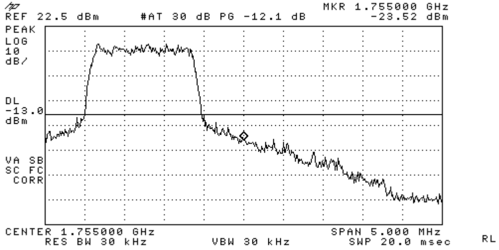
Figure 7-9 AWS 1700 Upper Band Edge @ CH 875
