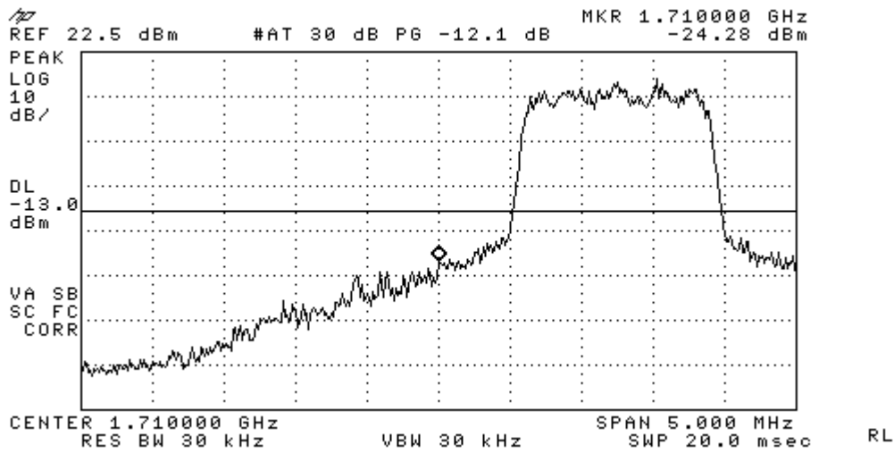
Figure 7-8 AWS 1700 Lower Band Edge @ CH 25
