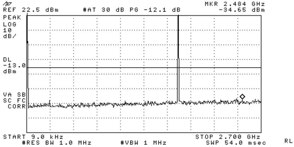
Figure 8-8a AWS 1700 - Conducted Spurious Emission (CH 450)
