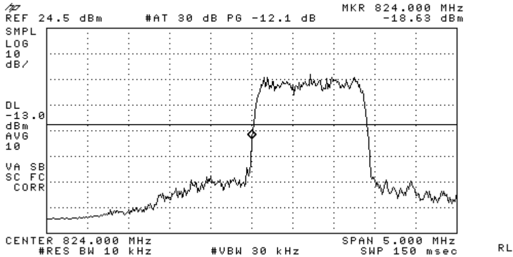
Figure 7-2 CDMA 800 Lower Band Edge @ CH 1013
