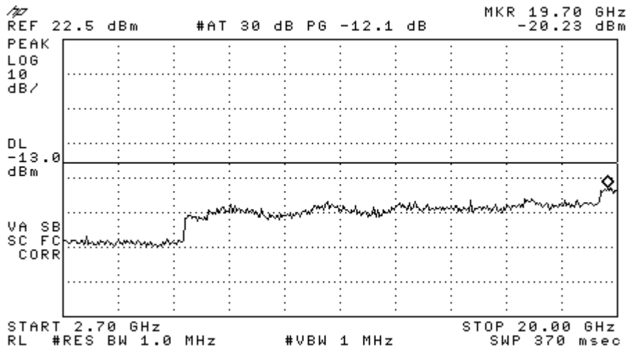
Figure 8-8b AWS 1700 - Conducted Spurious Emission (CH 450)
