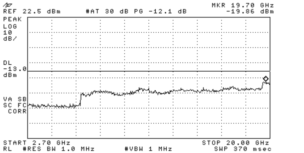
Figure 8-7b AWS 1700 - Conducted Spurious Emission (CH 25)
