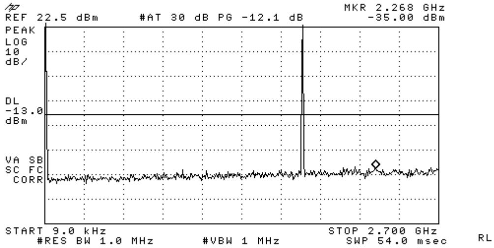
Figure 8-9a AWS 1700 - Conducted Spurious Emission (CH 875)
