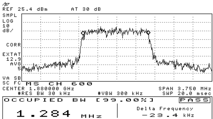
Figure 7-4 CDMA 1900 @ CH 600
