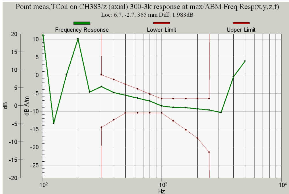
Figure 10.2b CDMA 800 Channel 383 Frequency Response
