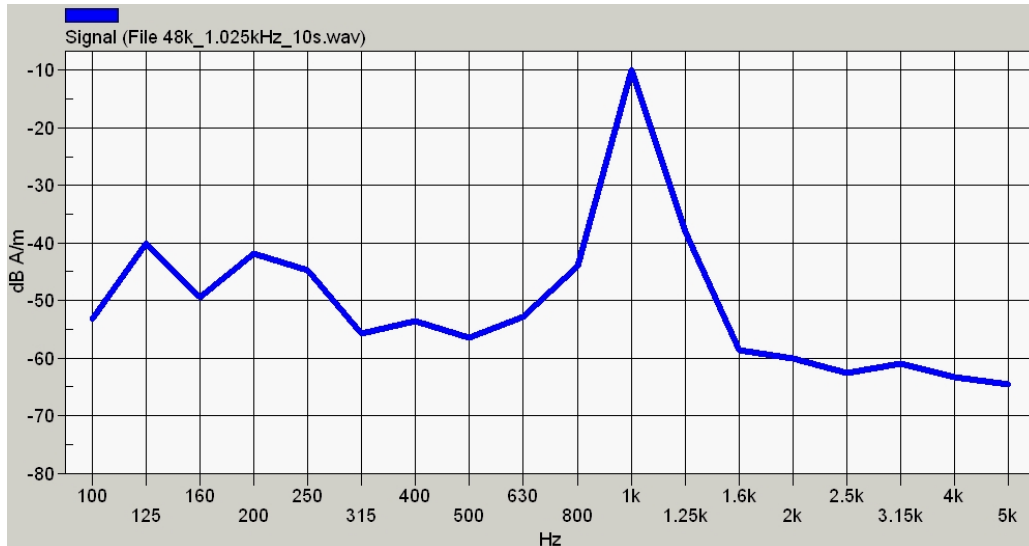
Figure 7.2a 1.025 KHz Voice signal spectrum
