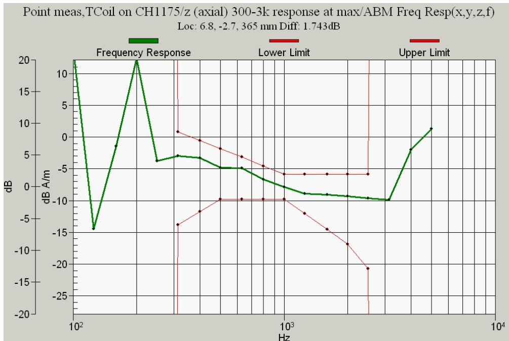
Figure 10.2e CDMA 1900 Channel 1175 Frequency Response
