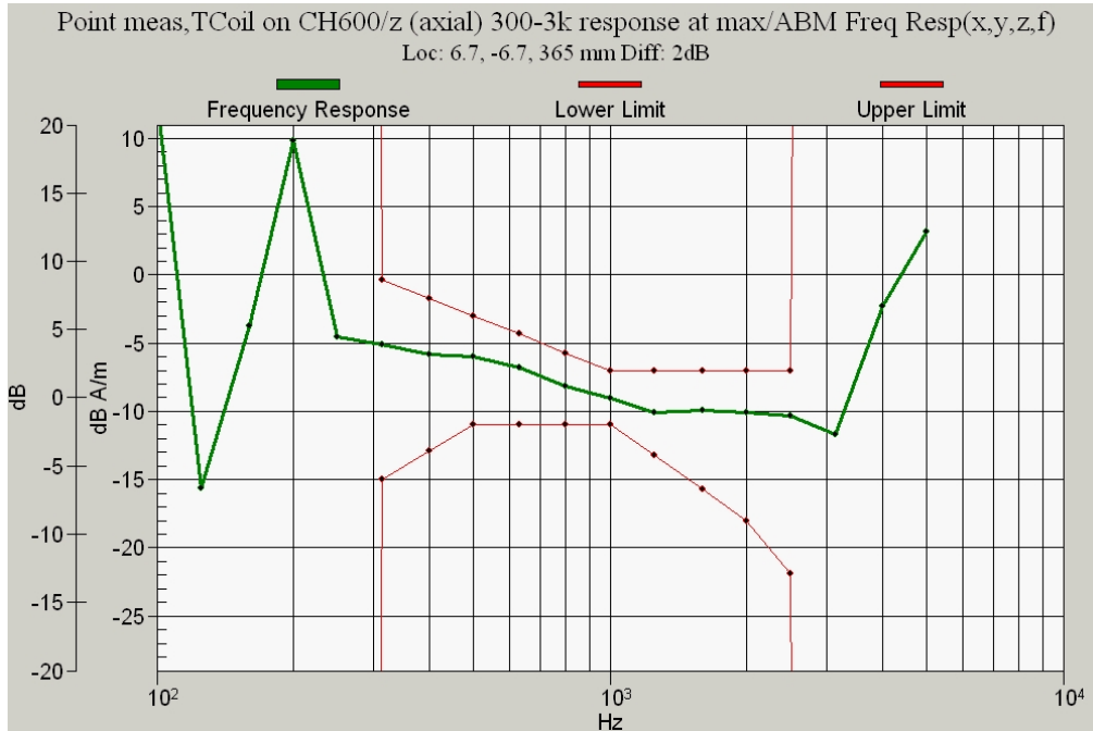
Figure 10.2e CDMA 1900 Channel 600 Frequency Response
