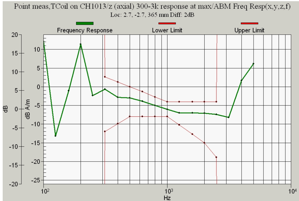
Figure 10.2a CDMA 800 Channel 1013 Frequency Response
