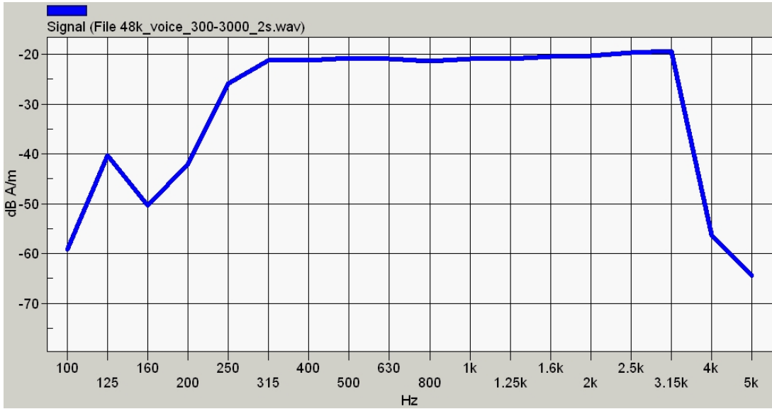
Figure 7.2b Broadband signal spectrum
