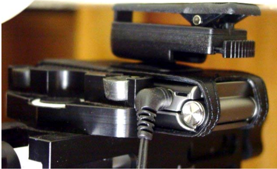
Figure 9E.5 Body SAR Phone setup Flip Closed with Leather Case (CV90-P0323-01)
