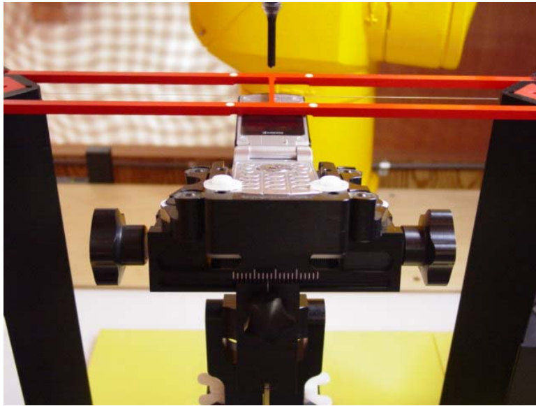
Figure 1a – RF Emission Test Setup
