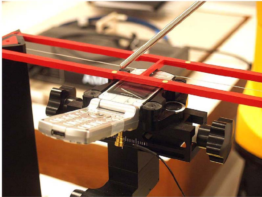
Figure 1c – T-coil Test Setup
