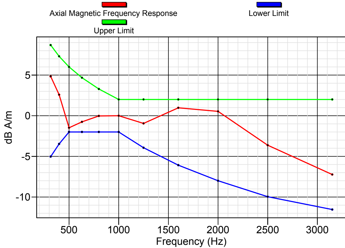
Frequency Response CDMA 800
