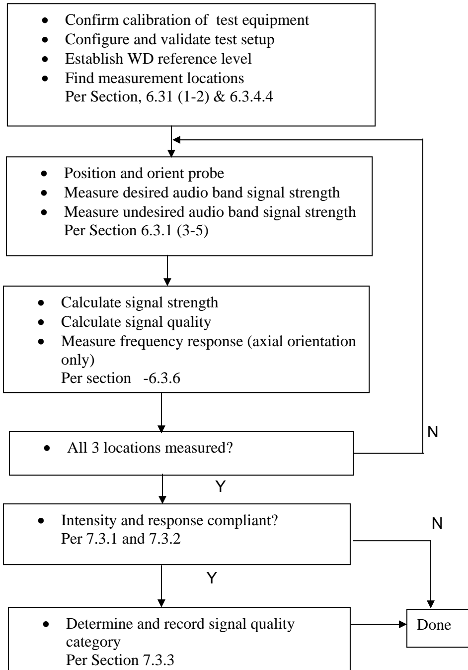
ANSI-C63.19-2006/5 test procedure sequence
