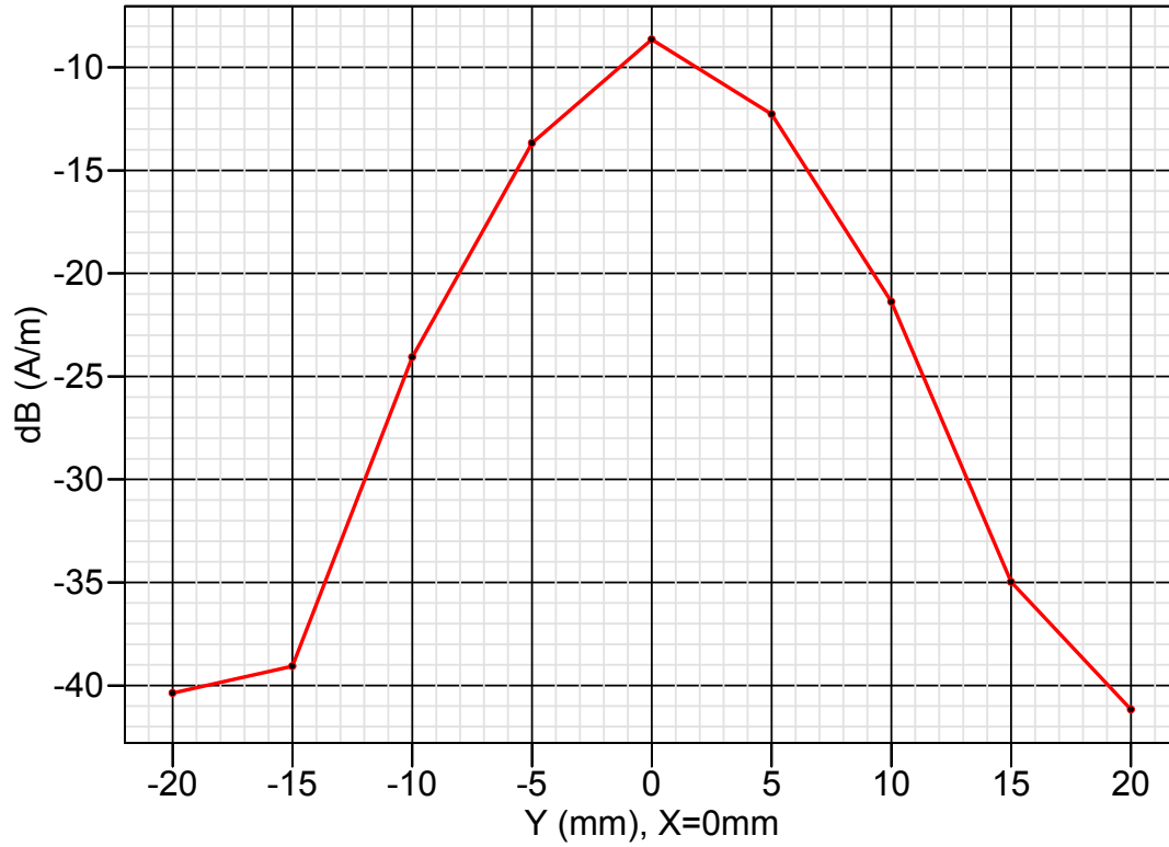
Axial Field Distribution
