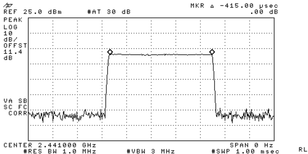
Figure 5. Duration of one transmission (Channels 39).
