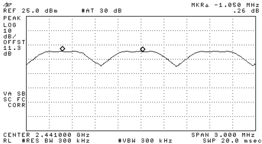
Figure 3. Carrier Frequency Separation between channels 38, 39 (mid-channel) & 40.
