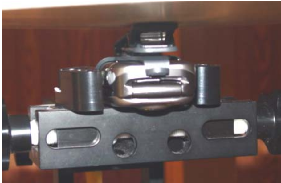
Figure 12.4 body SAR setup closed (with holster)
