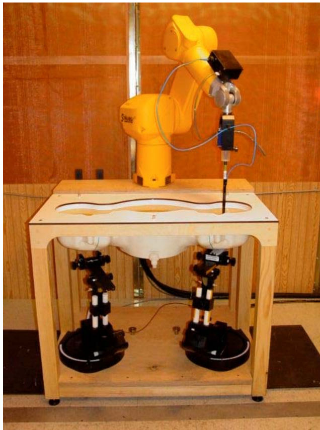
Figure 10.1 DASY 3 System
