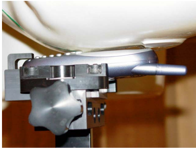
Figure 10.2 phone against the head (left cheek position)
