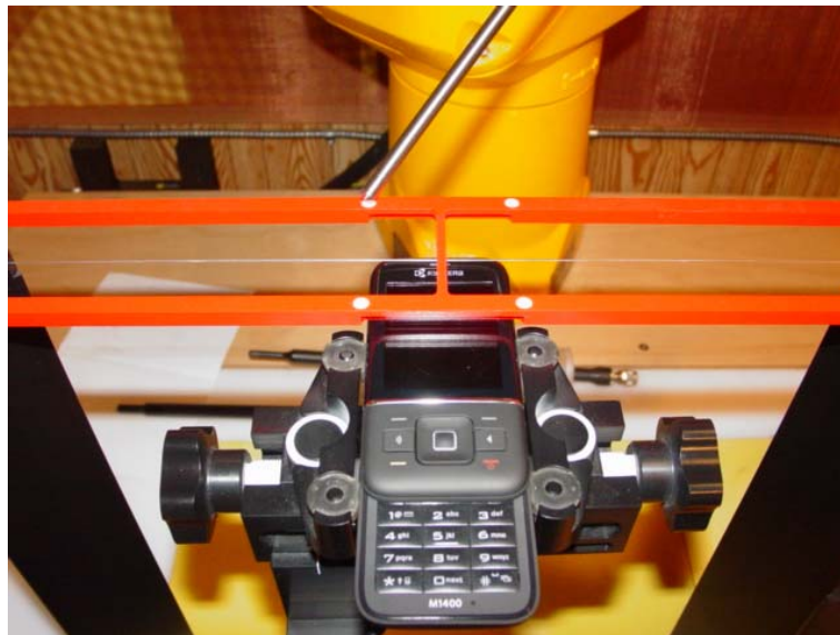
Figure 2b - HAC T-Coil Test Setup for Open Configuration
