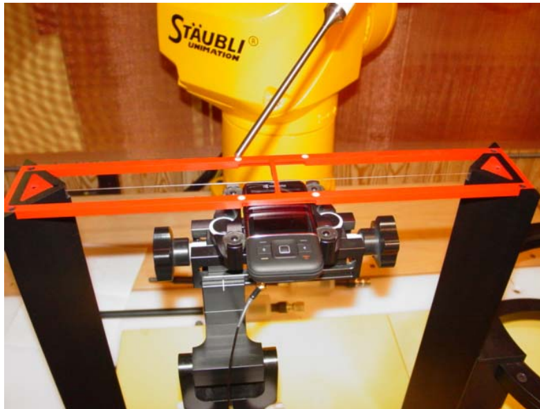
Figure 1a - HAC T-Coil Test Setup for Close Configuration
