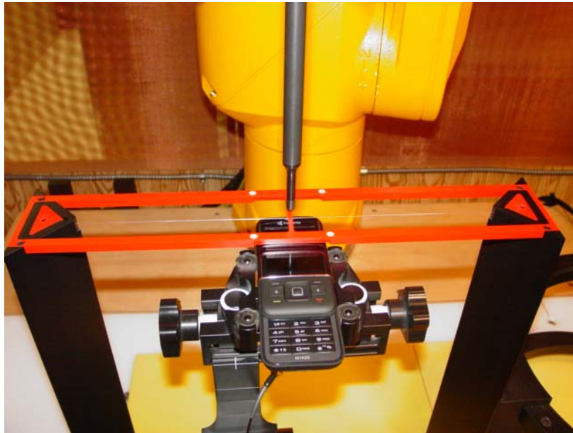
Figure 2a – HAC RF Emission Test Setup for Open Configuration
