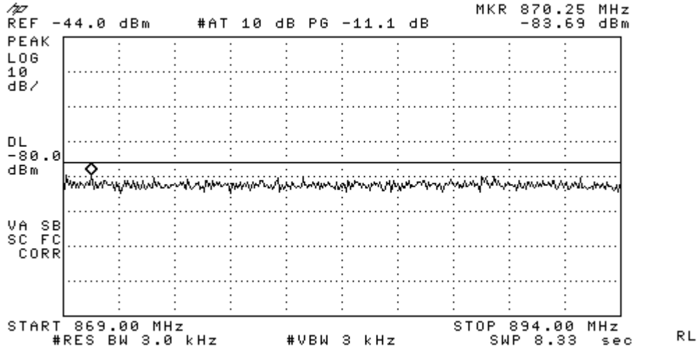
Figure 7-10 CDMA 800 - Emissions in base station frequency range (CH 1013)
