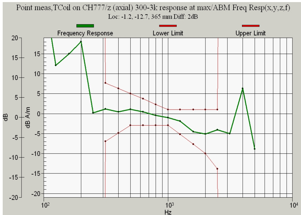
Figure 10.2c CDMA 800 Channel 777 Frequency Response
