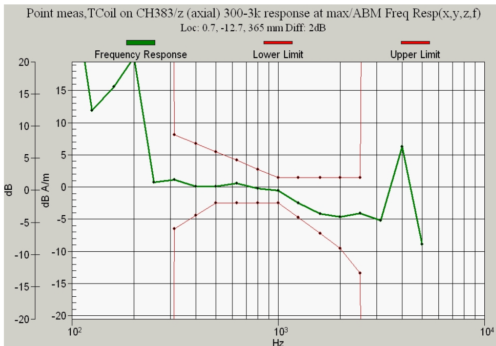
Figure 10.2b CDMA 800 Channel 383 Frequency Response
