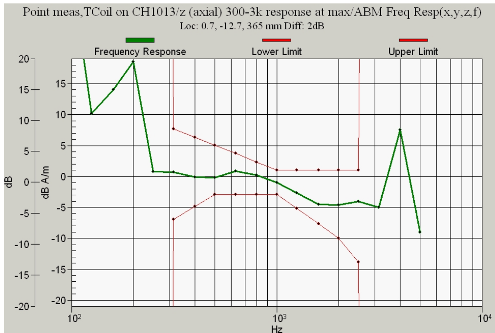
Figure 10.2a CDMA 800 Channel 1013 Frequency Response
