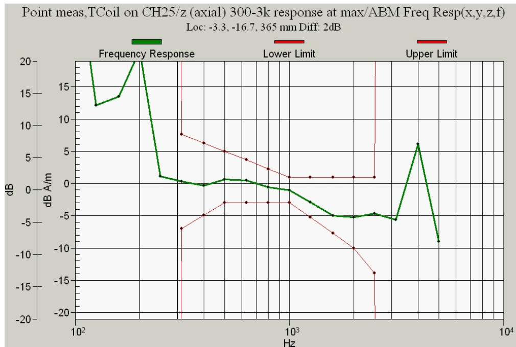
Figure 10.2d CDMA 1900 Channel 25 Frequency Response
