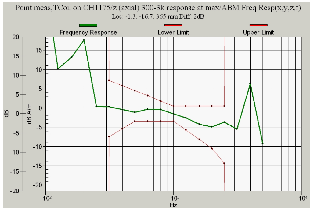
Figure 10.2e CDMA 1900 Channel 1175 Frequency Response
