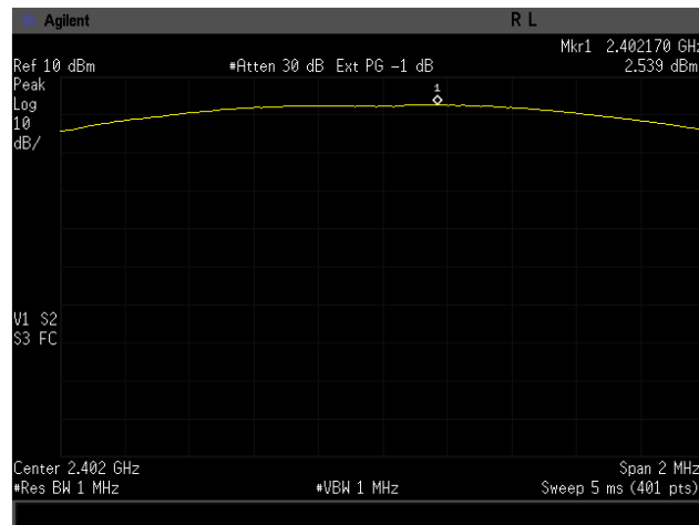
Figure 5-1a: Peak Output Power, EDR DQPSK Channel 0.
