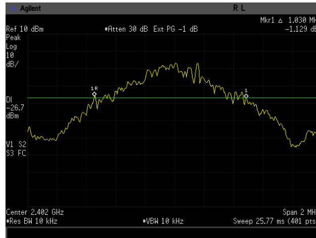
Figure 6-1a: 20dB Bandwidth Basic rate, Channel 0.
