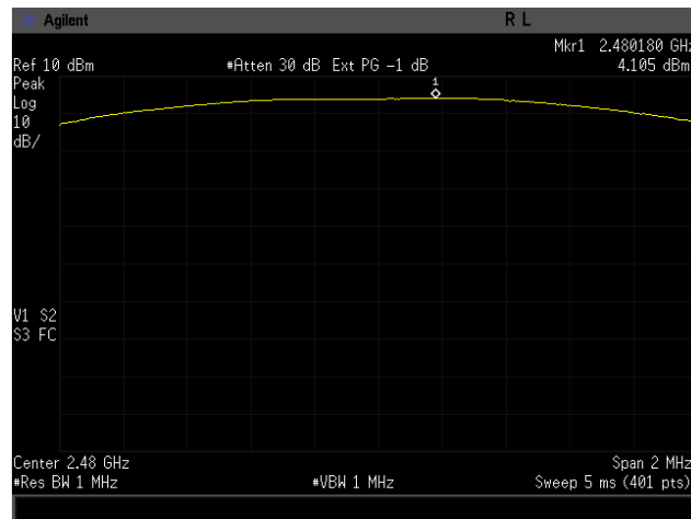
Figure 5-3a: Peak Output Power, EDR DQPSK Channel 78.
