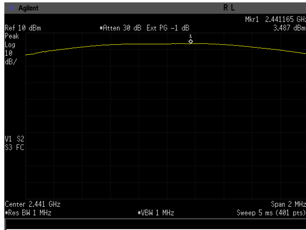
Figure 5-2a: Peak Output Power, EDR DQPSK Channel 39.
