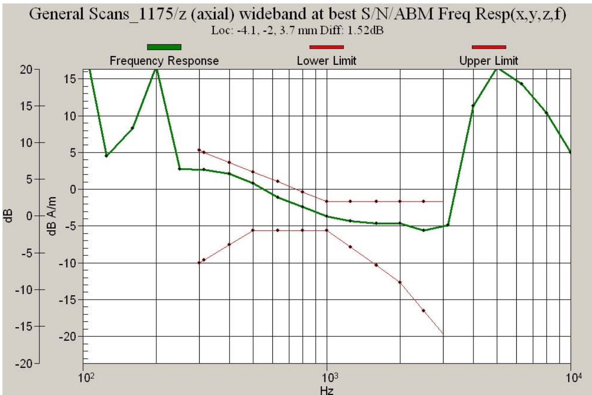
Figure 10.2c CDMA 1900 Channel 1175 Frequency Response
