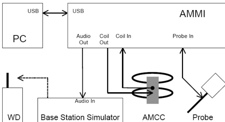
Figure 5.2b Setup Cabling
