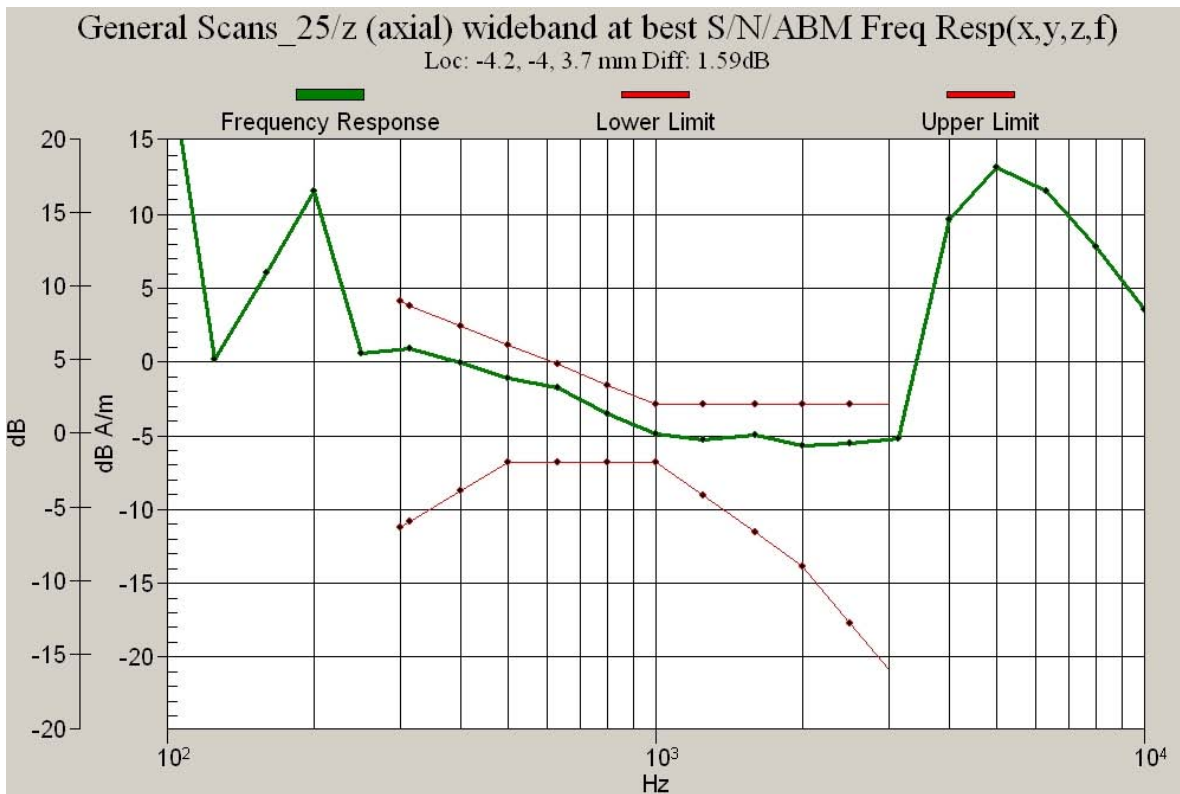
Figure 10.2a CDMA 1900 Channel 25 Frequency Response
