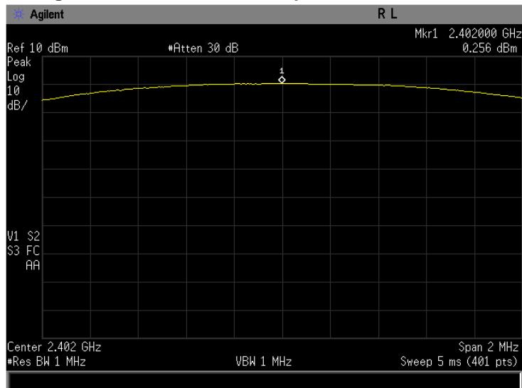
Figure 7-1c: EDR 3 Peak Output Power, Channel 0.
