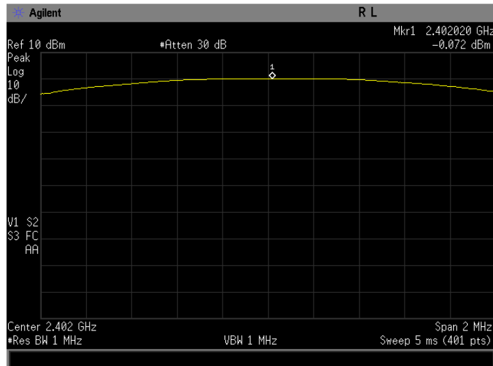
Figure 7-1b: EDR 2 Peak Output Power, Channel 0.
