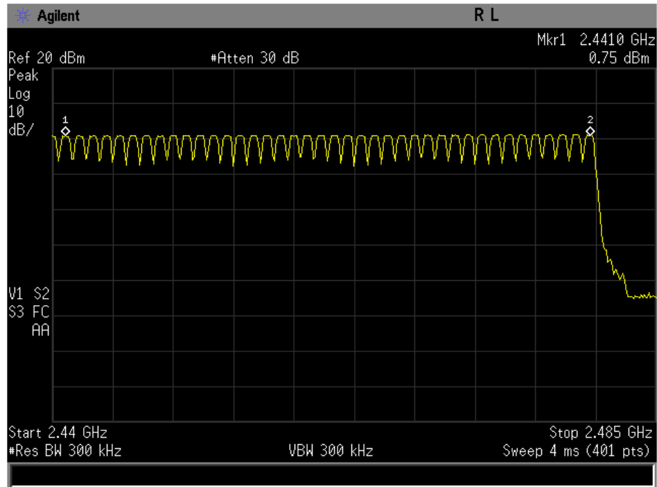
Figure 5b: Number of Hopping Frequencies (Channels 39-78)
