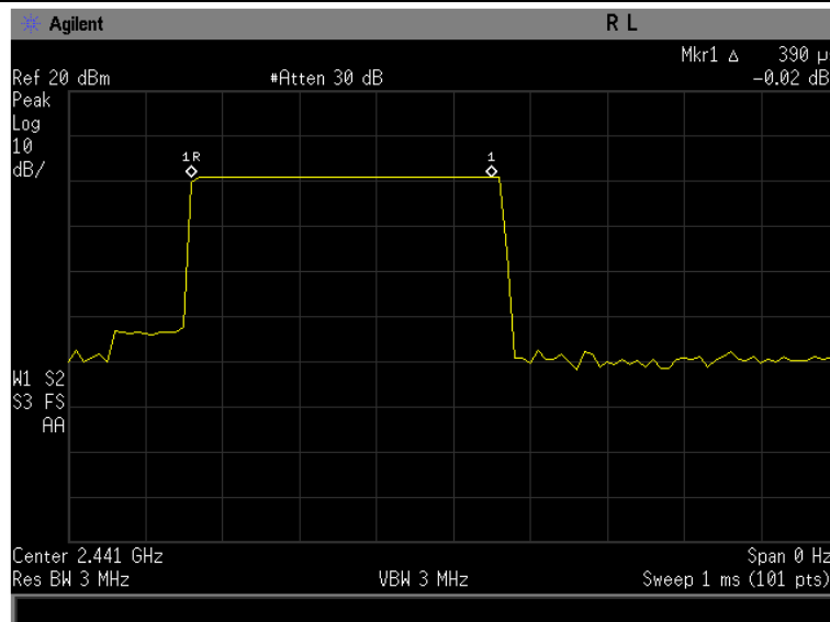
Figure 6: Duration of one transmission (Channel 39)
