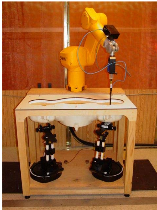
Figure 7.1 DASY 4 System
