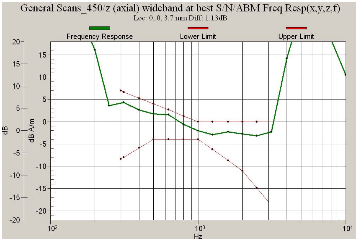
Figure 10.2b CDMA 1700 Channel 450 Frequency Response
