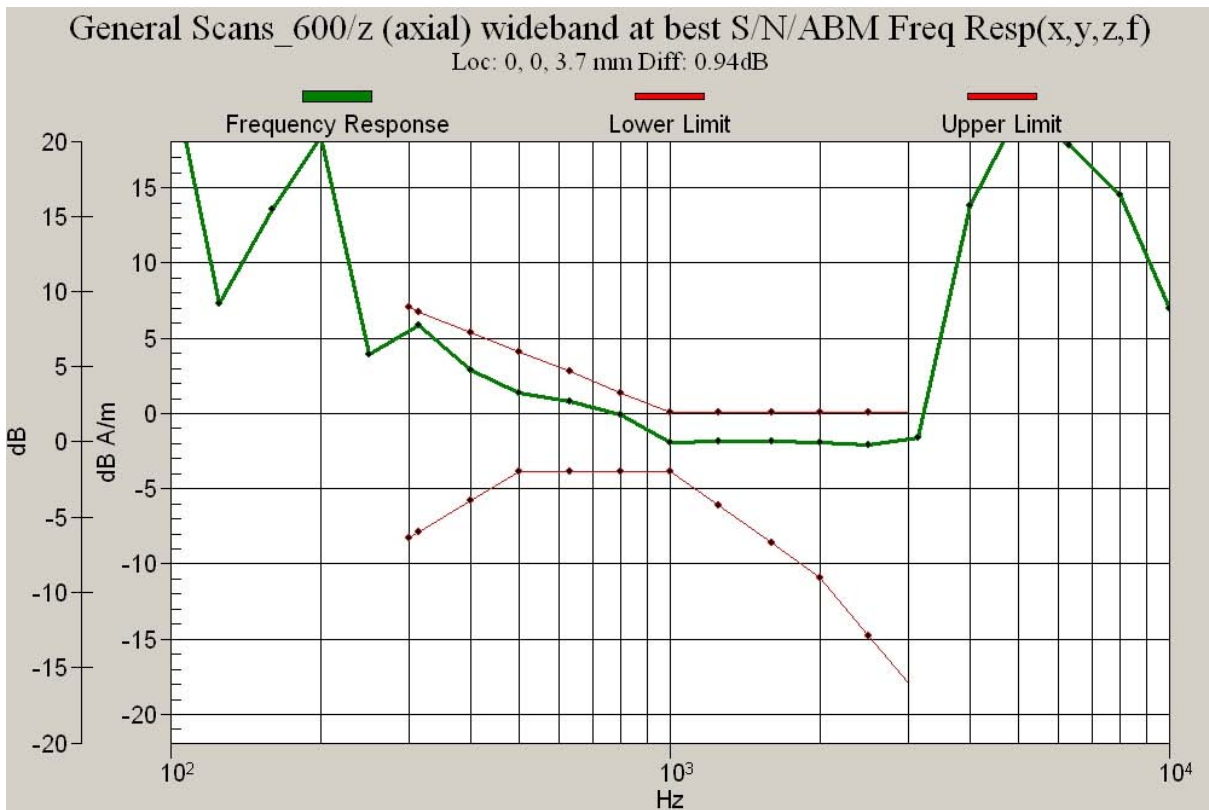
Figure 10.2c CDMA 1900 Channel 600 Frequency Response
