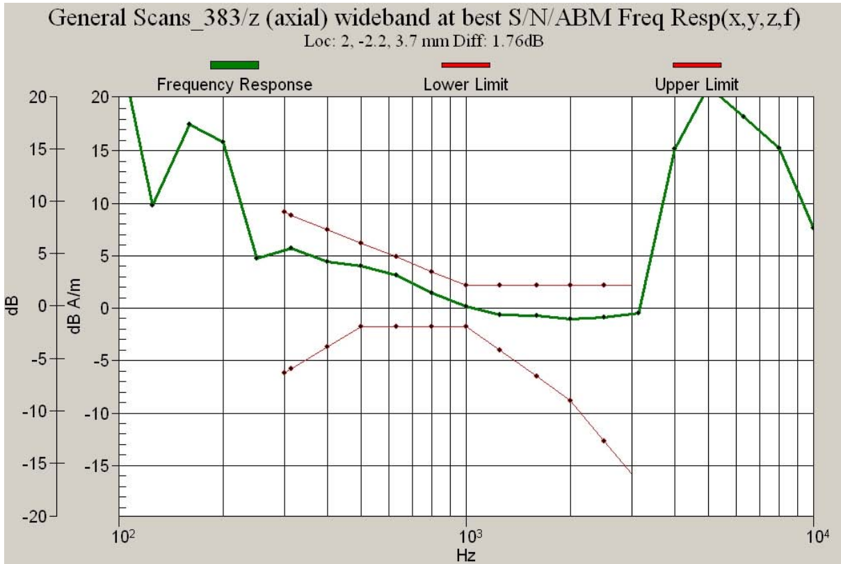
Figure 10.2a CDMA 800 Channel 383 Frequency Response
