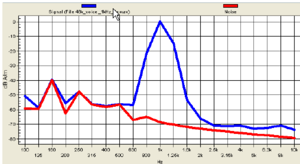
Figure 7.2a 1 kHz Voice signal spectrum
