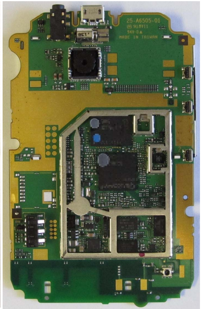
New PWB
