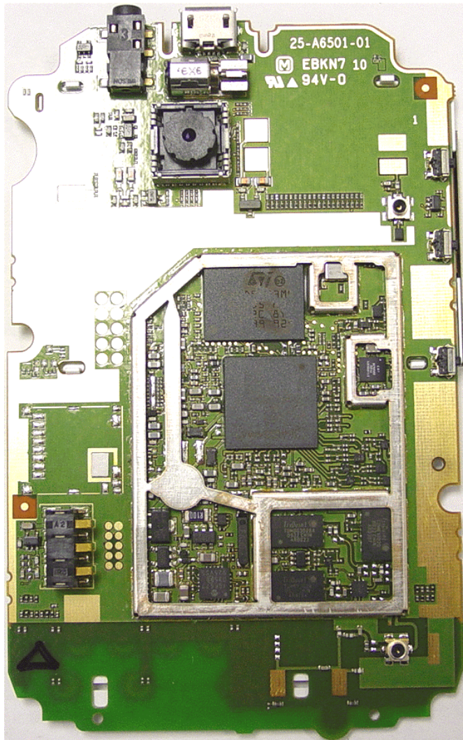
Original PWB
