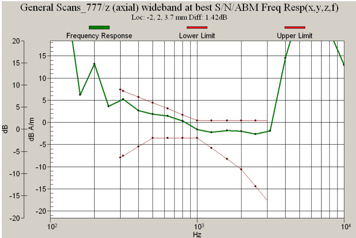
Figure 10.2a CDMA 800 Channel 777 Frequency Response
