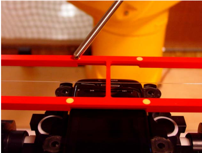
Figure 1a - HAC T-Coil Test Setup for Closed Configuration
