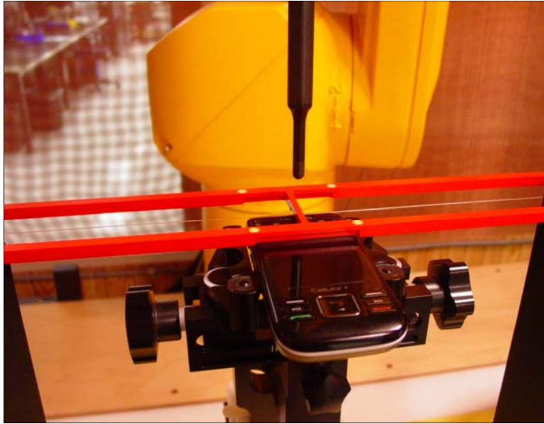
Figure 1a – HAC RF Emission Test Setup for Closed Configuration
